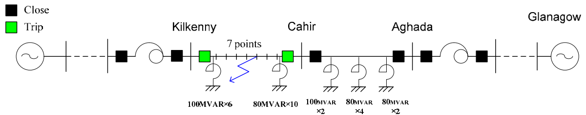
Fig. 5-27 Compensation of 400 kV Kilkenney – Cahir – Aghada line in Case B5 (approx. 50 % compensation).
