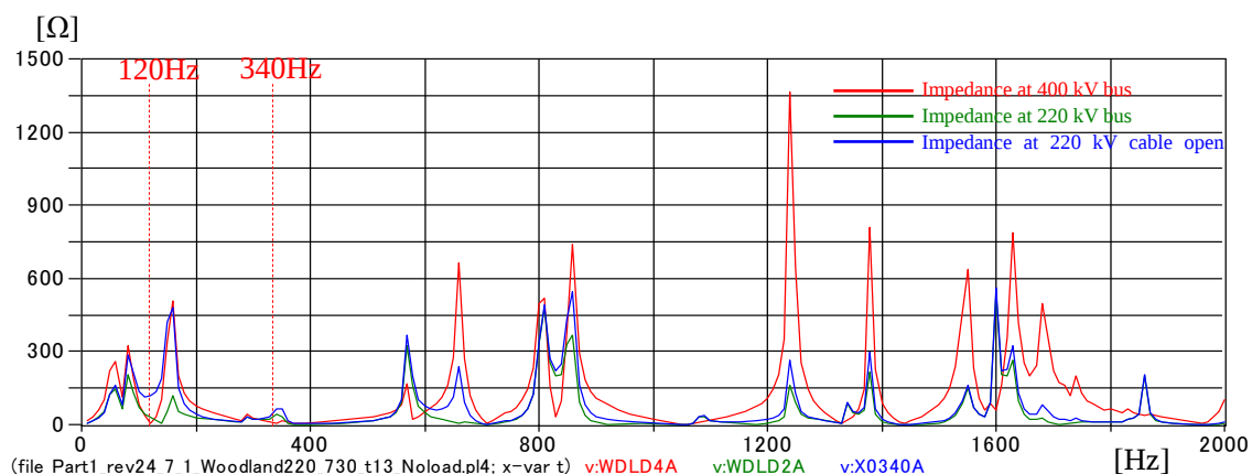
Fig. A1-40 Frequency scan at the Woodland 400 kV and 220 kV buses and 220 kV cable open end (phase to earth).
