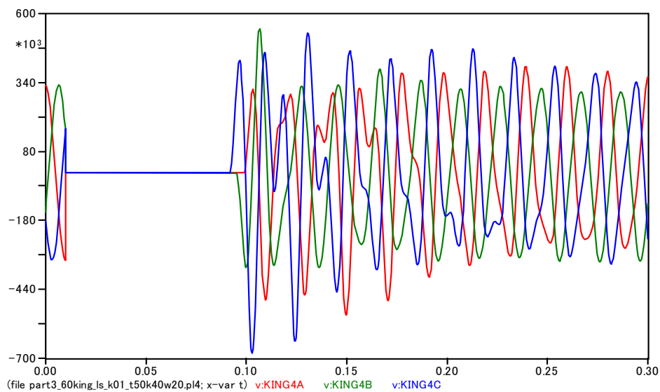
Fig. 4.20 Overvoltage caused by islanding under largest impedance value of Turleenan. (Dummy source impedance at Turleenan 275 kV: 50 mH)
