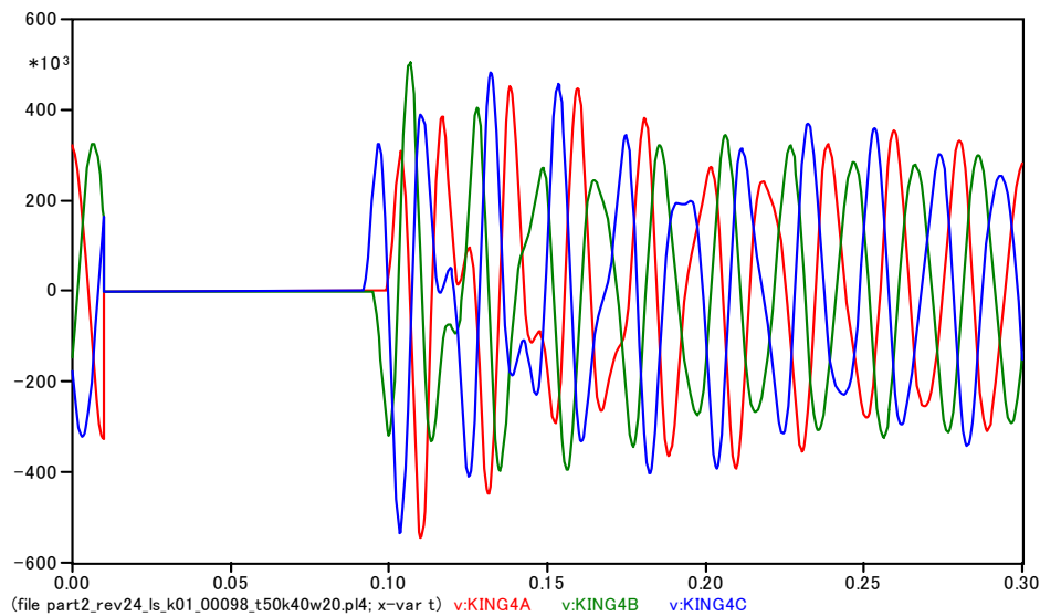
Fig. 4.34 Overvoltage caused by islanding under largest impedance value of Turleenan. (dummy source impedance at Turleenan 275 kV: 50 mH)
