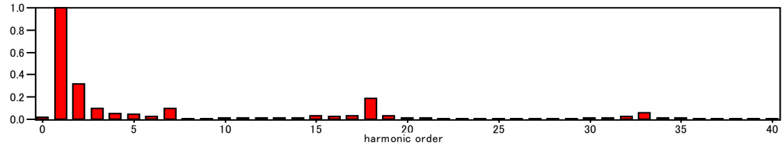
Fig. A2-48 Frequency component spectrum of the switching waveform at Woodland 220 kV bus (phase to earth).
