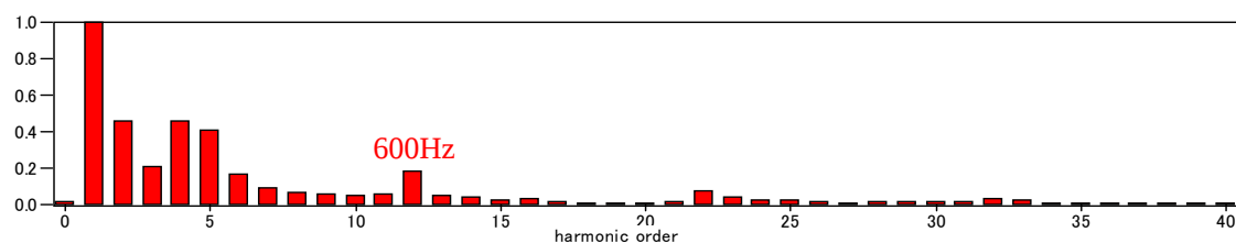
Fig. A1-29 Frequency component spectrum of the switching waveform at the 220 kV cable open end (phase to earth).
