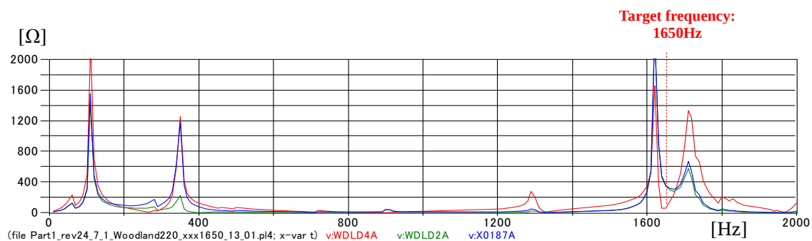
Fig. A2-45 Frequency scan at the Woodland 400 kV and 220 kV buses and 220 kV cable open end (phase to earth).
