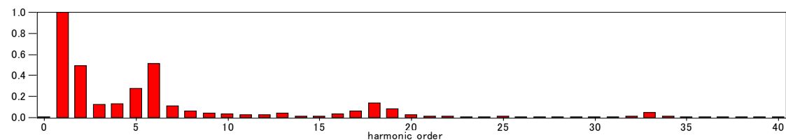
Fig. A1-4 Frequency component spectrum of the switching waveform at the 220 kV cable open end (phase to earth).
