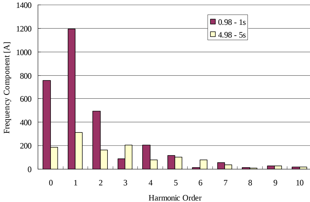
Fig. 4.13 Frequency components in transformer inrush current in Phase A.
