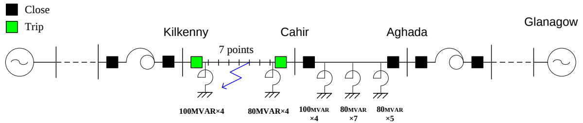
Fig. 5-25 Compensation of 400 kV Kilkenney – Cahir – Aghada line in Case B2 (Base case).
