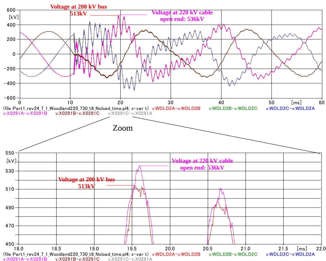
Fig. A1-7 Switching waveforms at the Woodland 220 kV bus and 220 kV cable open end (phase to phase).
