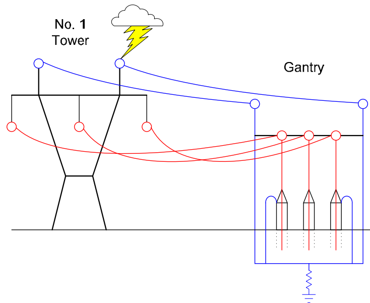
Fig. 6.1 Lightning overvoltage in metallic sheath.
