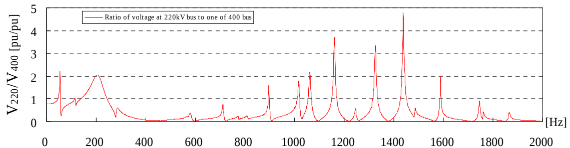
Fig. 4-6 Amplification ratio at Woodland.
