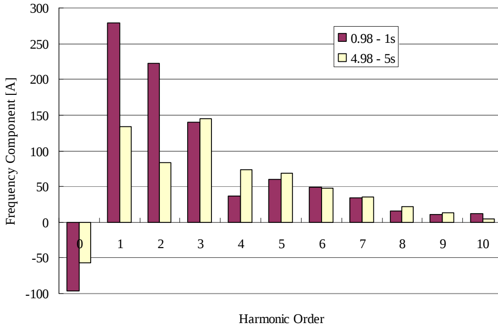
Fig. 4.14 Frequency components in transformer inrush current in Phase C.
