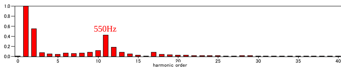
Fig. A1-19 Frequency component spectrum of the switching waveform at the 220 kV cable open end (phase to earth).
