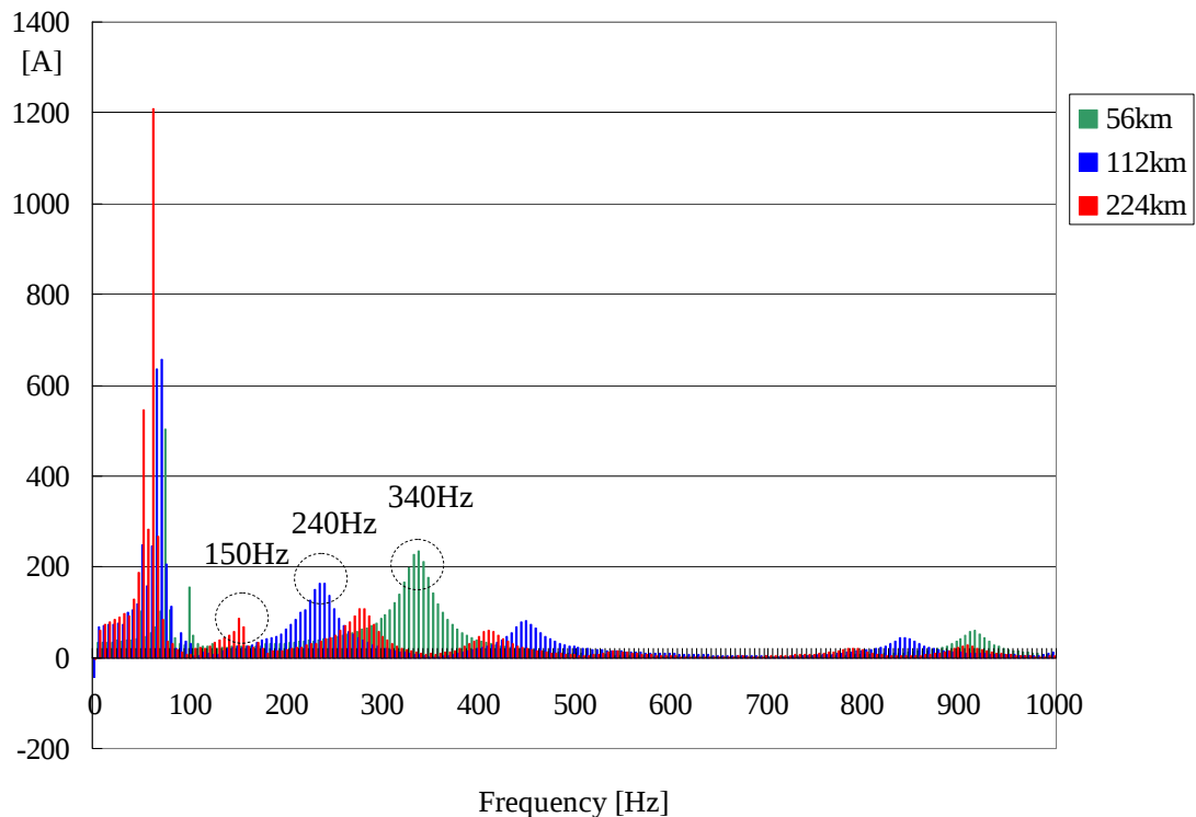
Fig. 4-74 Fourier transform of the line energisation overvoltage.
