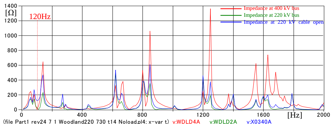
Fig. A1-45 Frequency scan at the Woodland 400 kV and 220 kV buses and the 220 kV cable open end (phase to earth).
