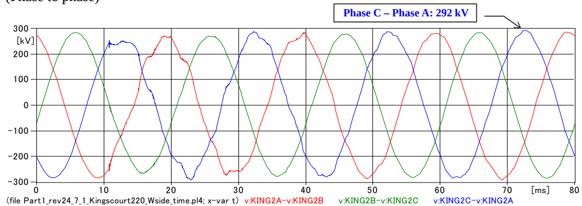
Fig. 4-47 Waveforms of the overvoltage at the Kingscourt 220kV bus (phase to phase).
