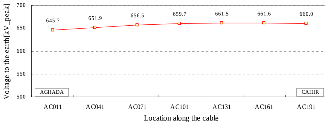
Fig. 4-100 Overvoltage caused by system islanding with 50 % cable length.
