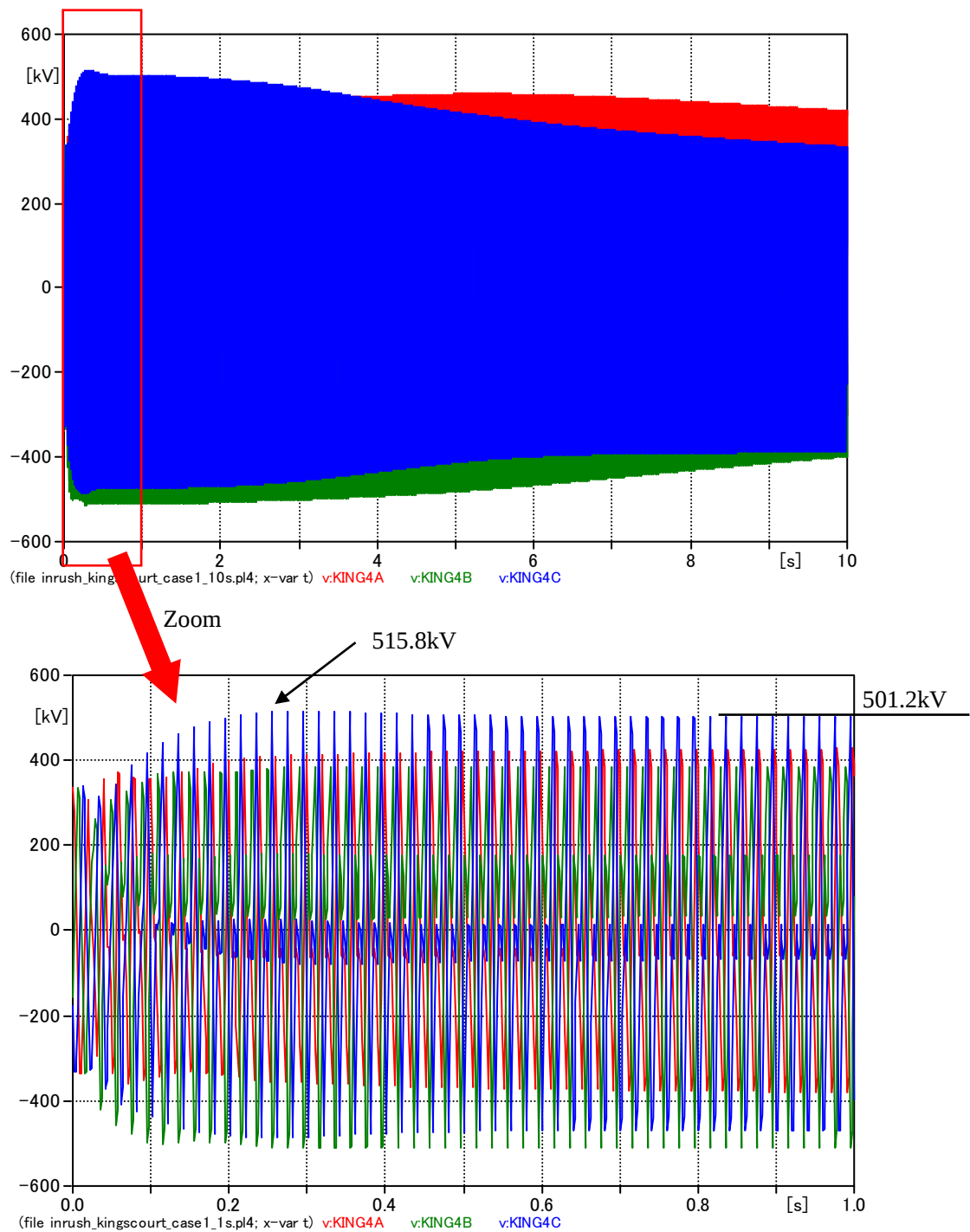
Fig. 4.23 Kingscourt 400 kV bus voltage in transformer inrush.
