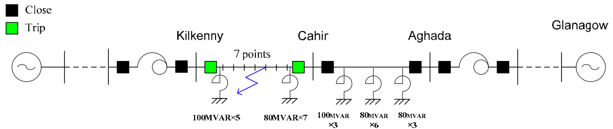
Fig. 5-26 Compensation of 400 kV Kilkenney – Cahir – Aghada line in Case B4 (approx. 75 % compensation).
