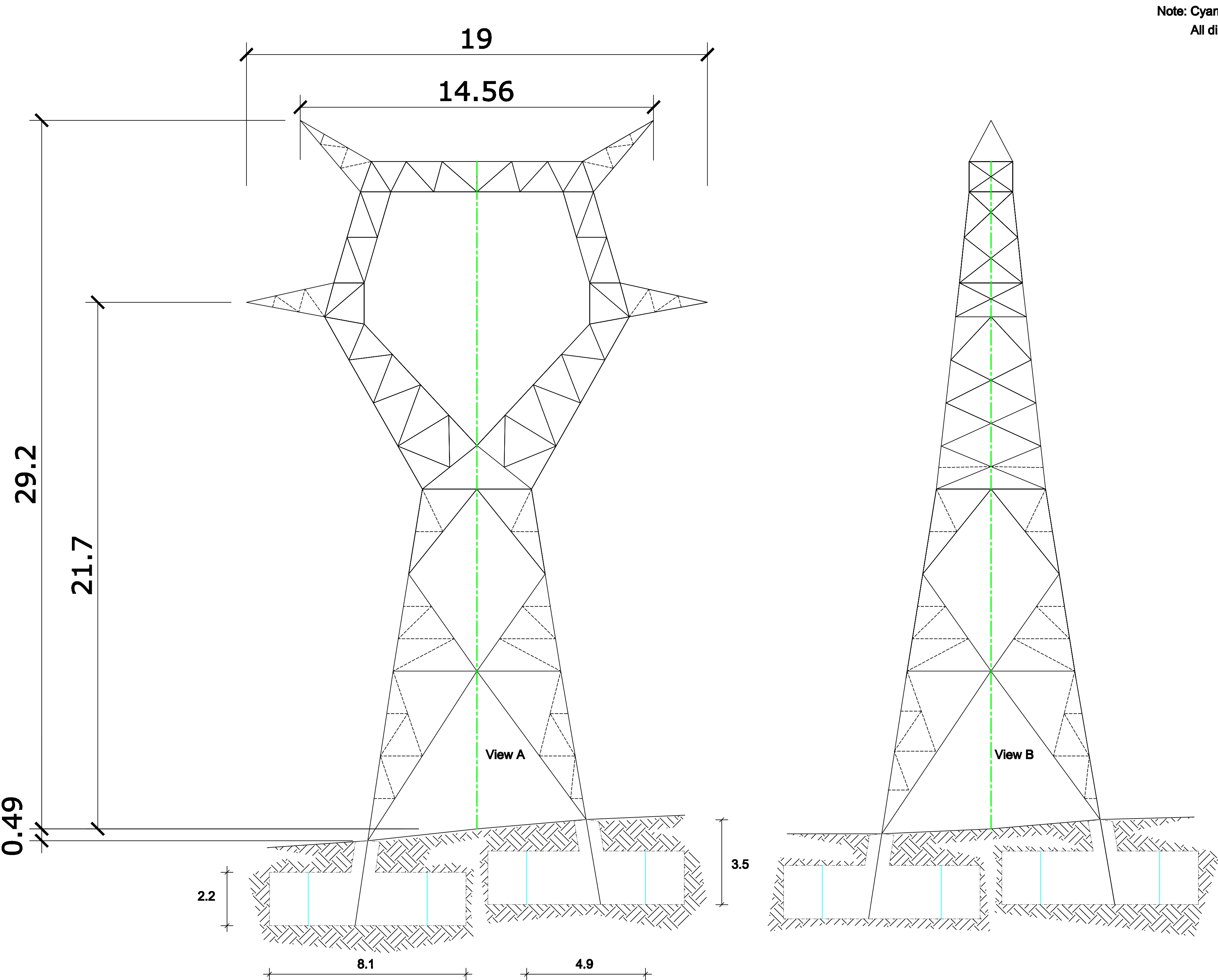
View 2: 1/100
