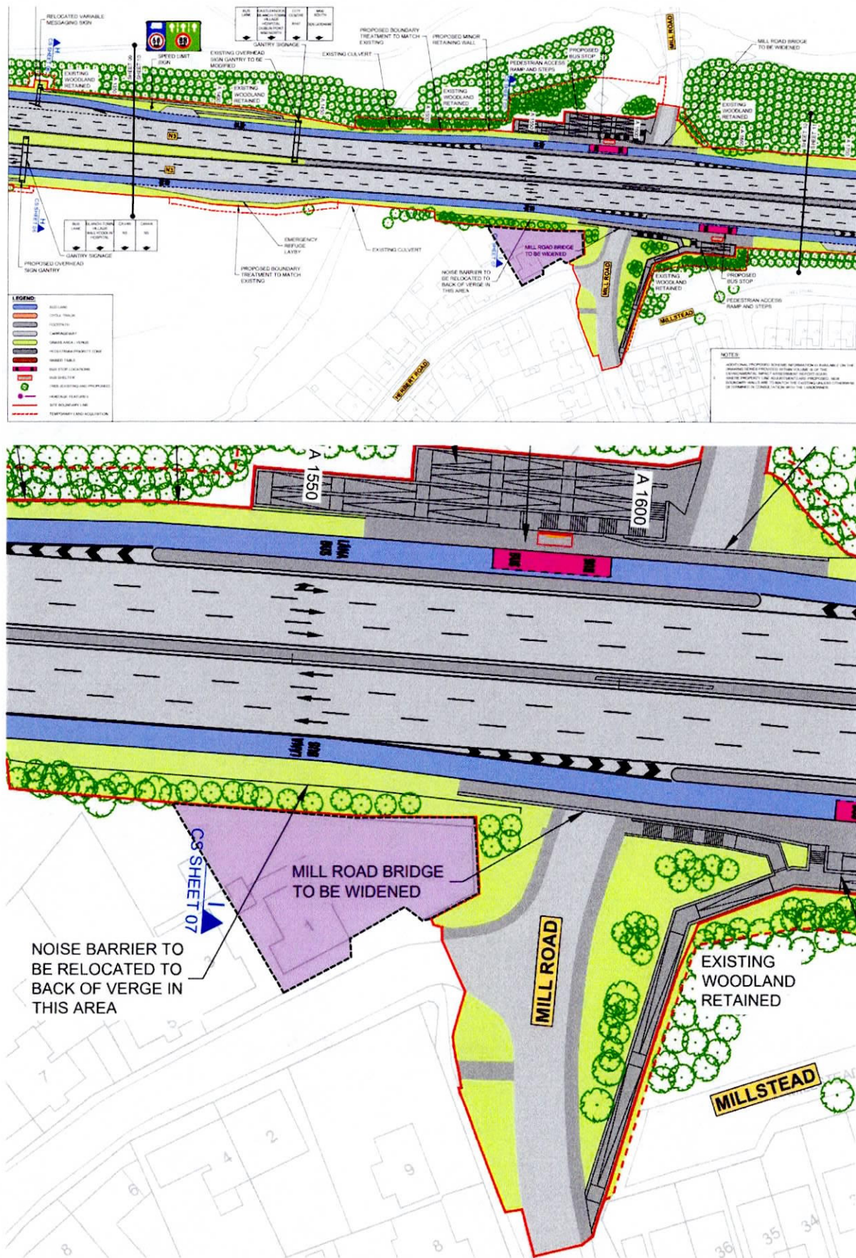
Figure 3.0 Extracts from Sheet 10 of the General Arrangement drawing illustrating the proposed works relative to our client's site (purple fill).
