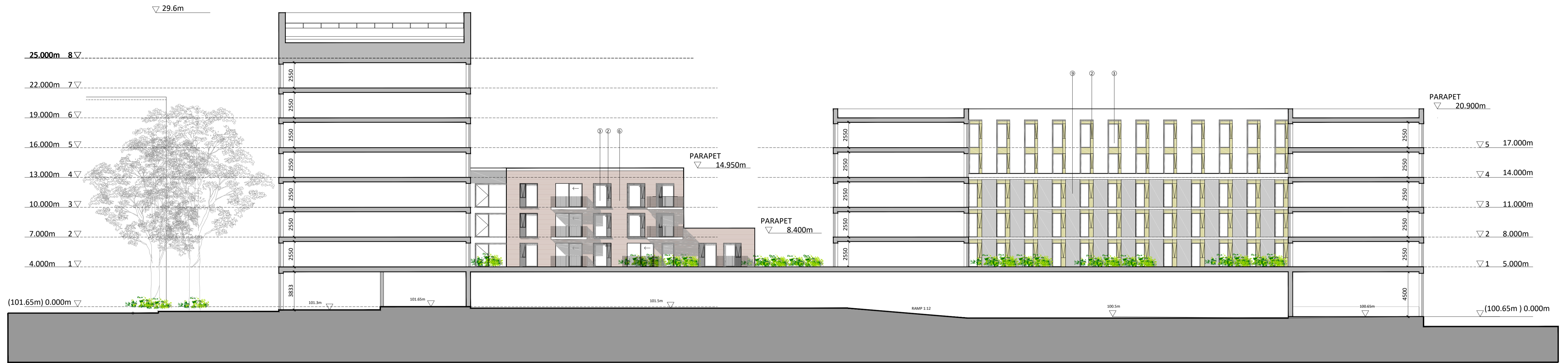
CONTEXTUAL SECTION ELEVATION SECTOR 2 & 3_LL SCALE 1:200
