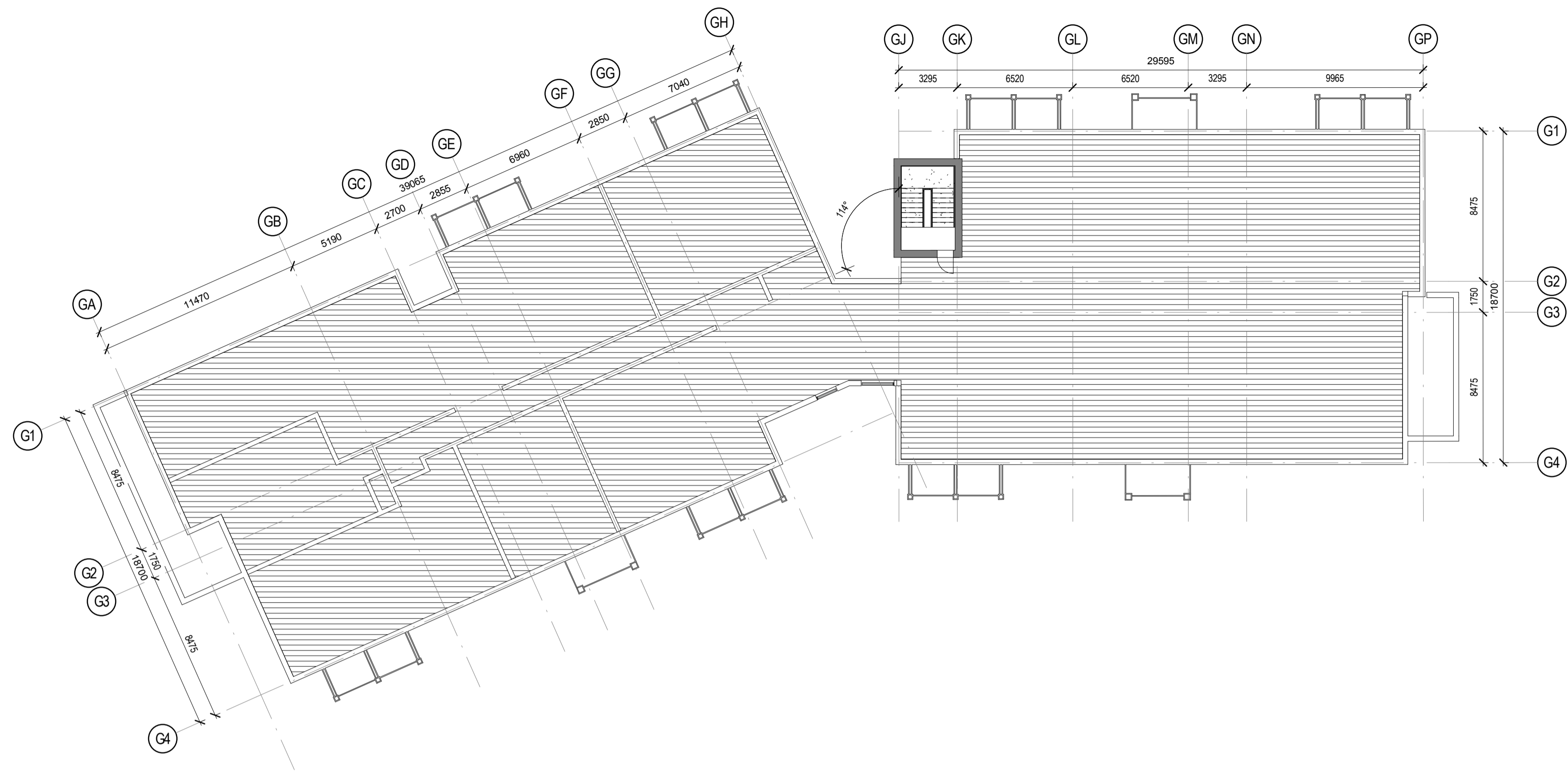
1 G_08_Roof Level 1 : 200
