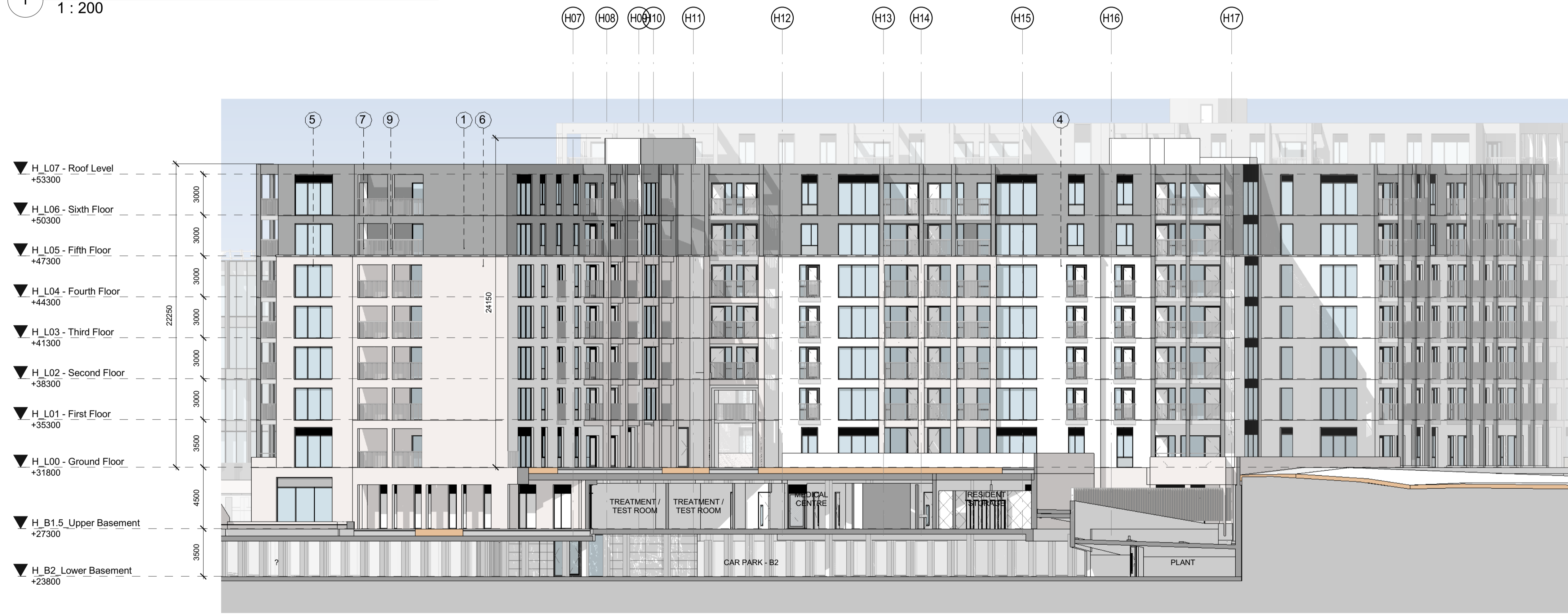
2 Block H_Facade 02_South_Planning 1 : 200
