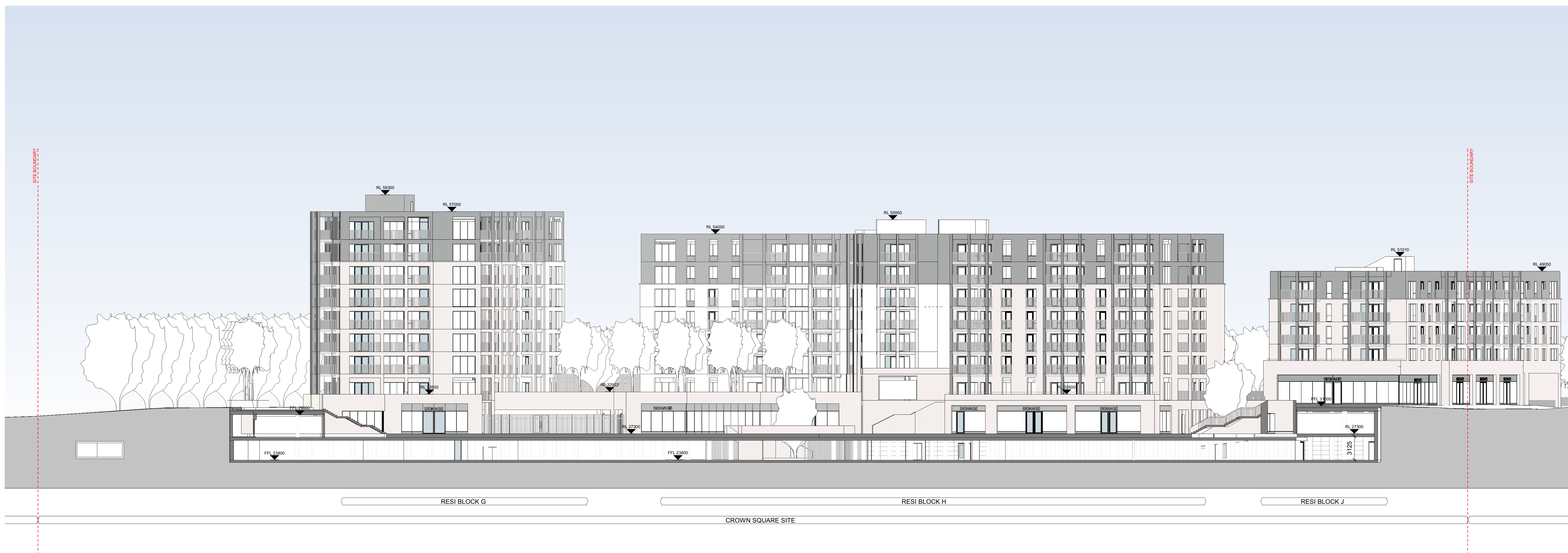
1 Site_Section 8_1.200 1:200
