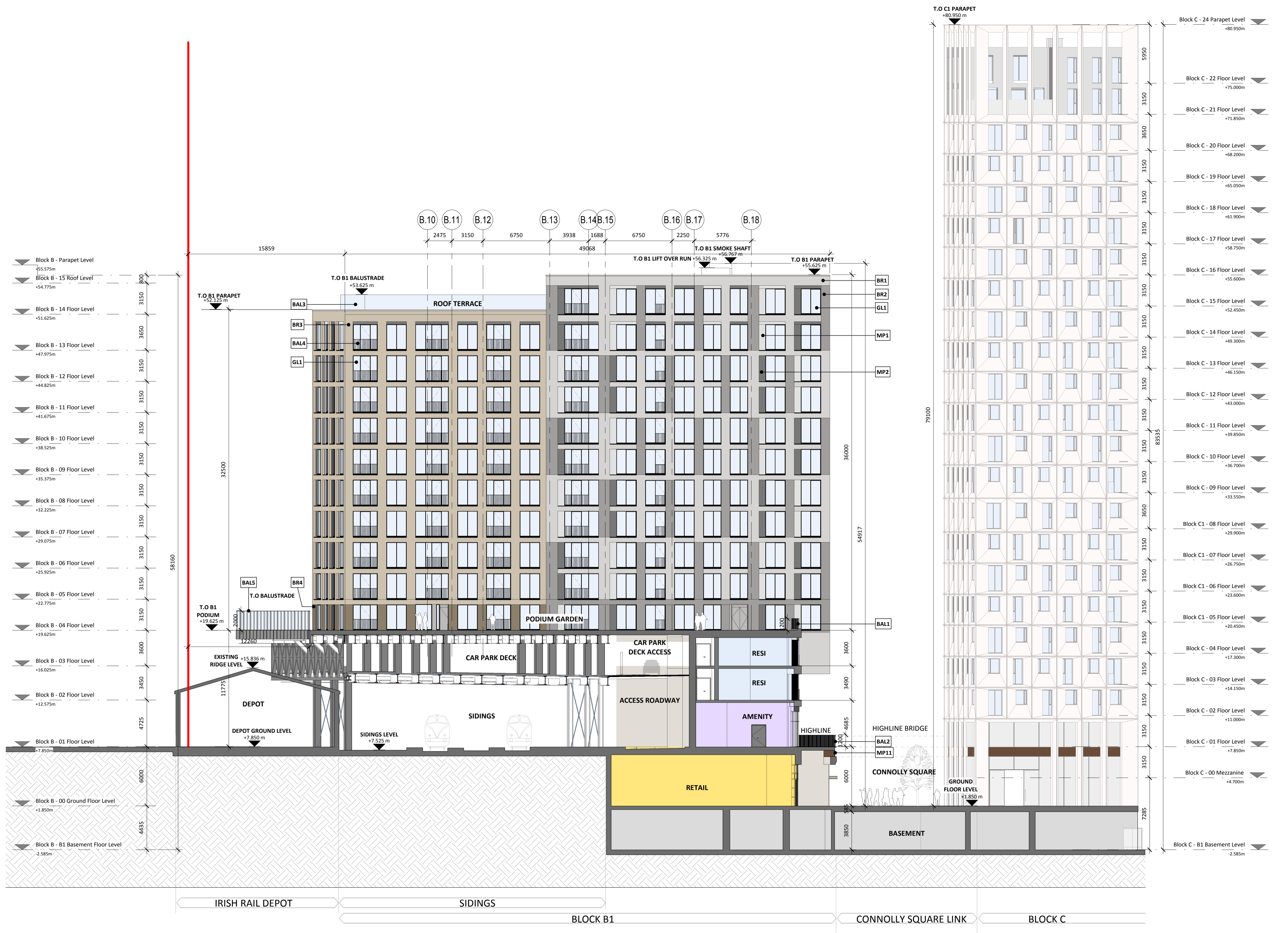
B-B BLOCK B - SECTION B-B 1 : 200
