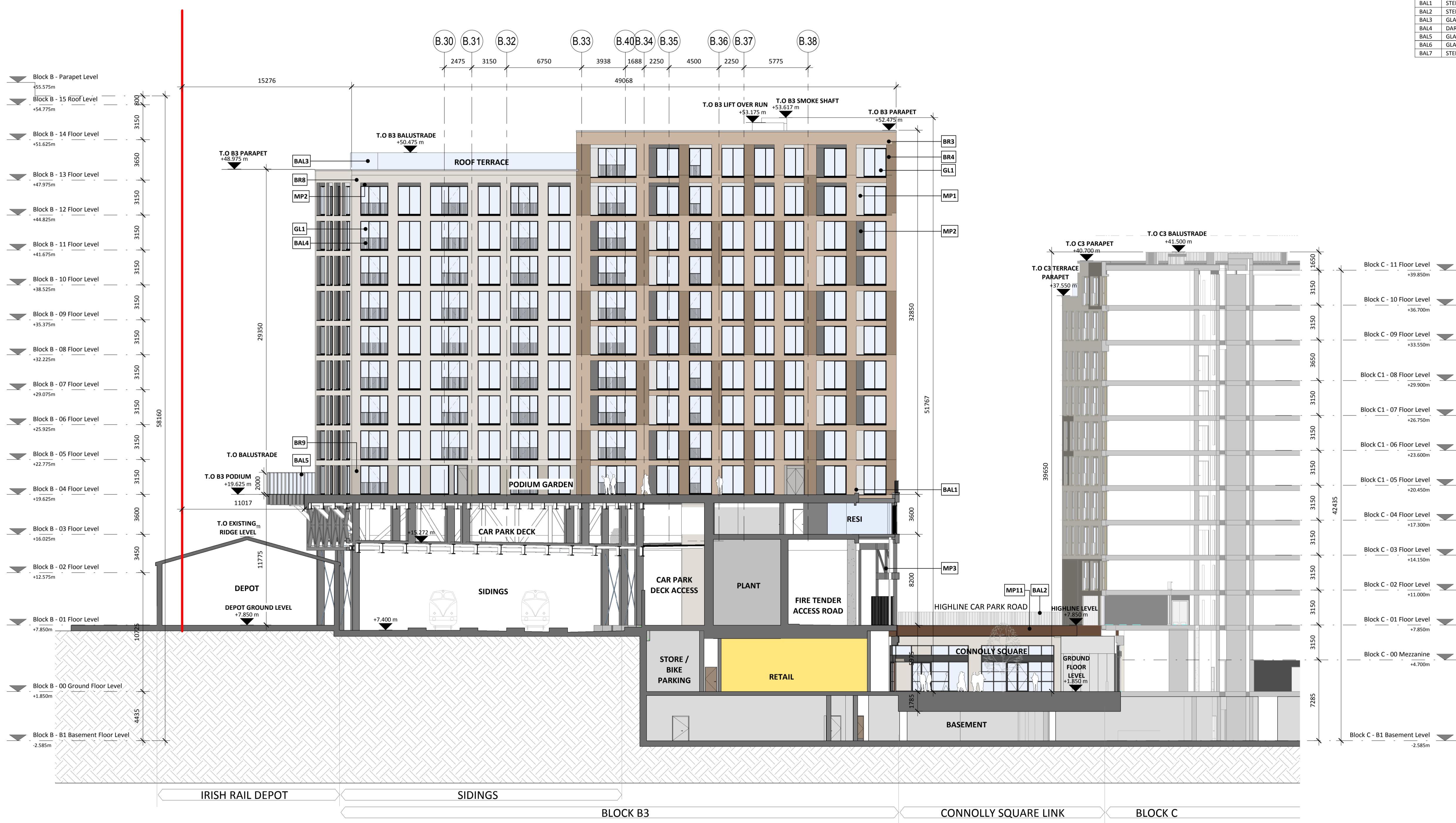
F-F BLOCK B - SECTION F-F 1 : 200
