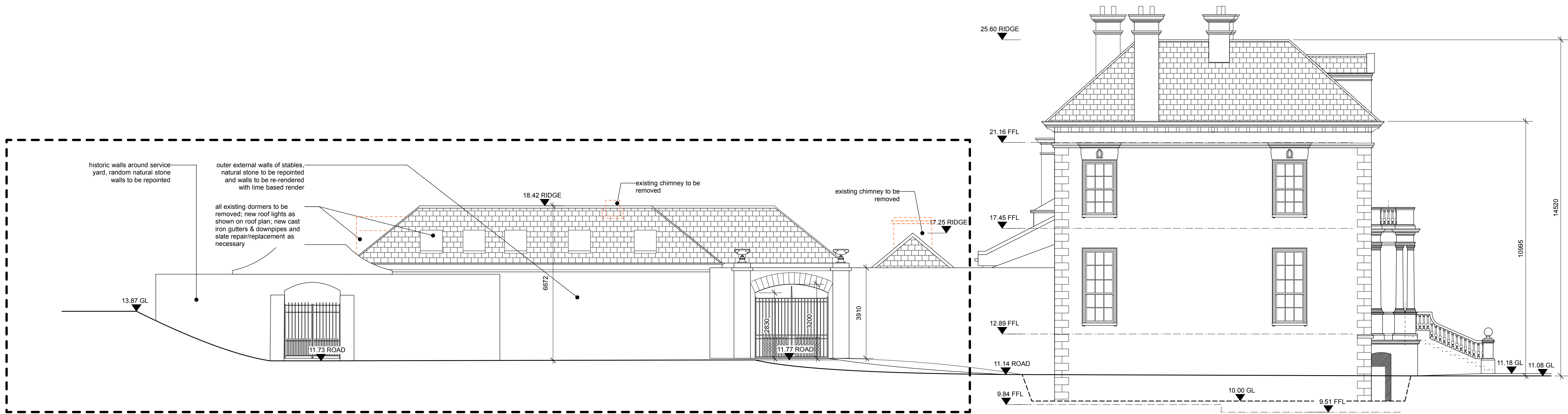
01 Proposed Side (South) Elevation 110 1:100
