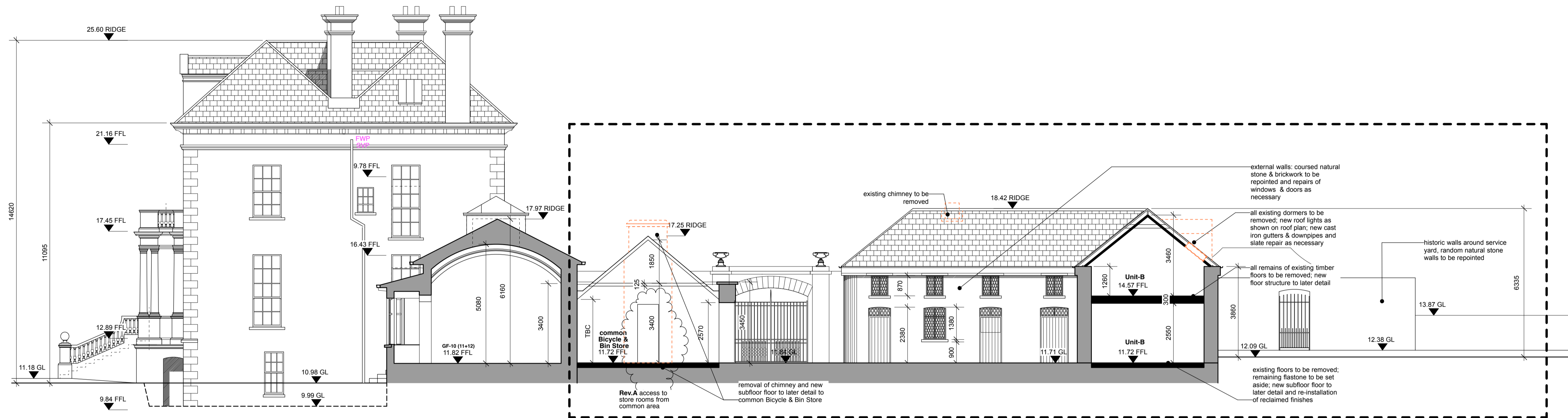
01 Proposed Section C-C 111 1:100
