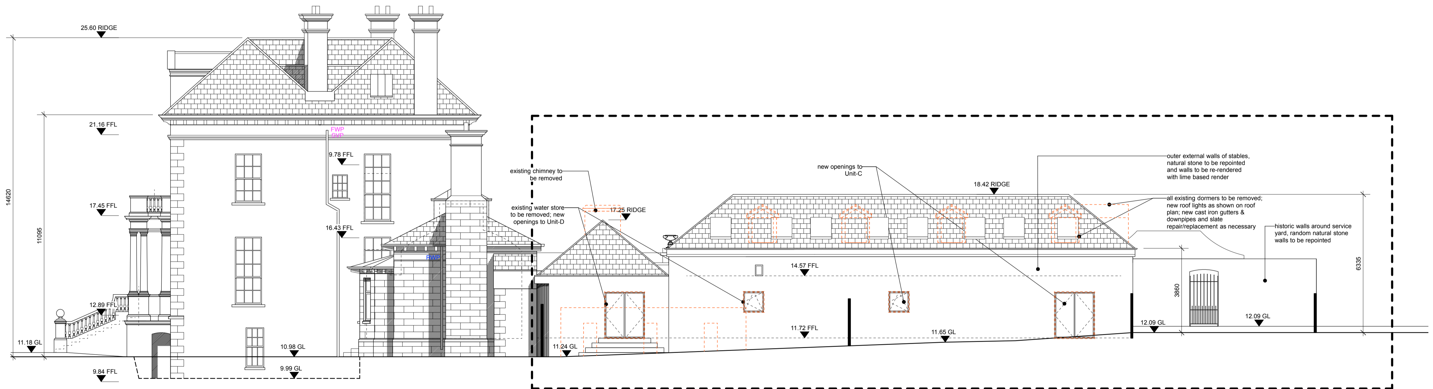
02 Proposed Side (North) Elevation 111 1:100
