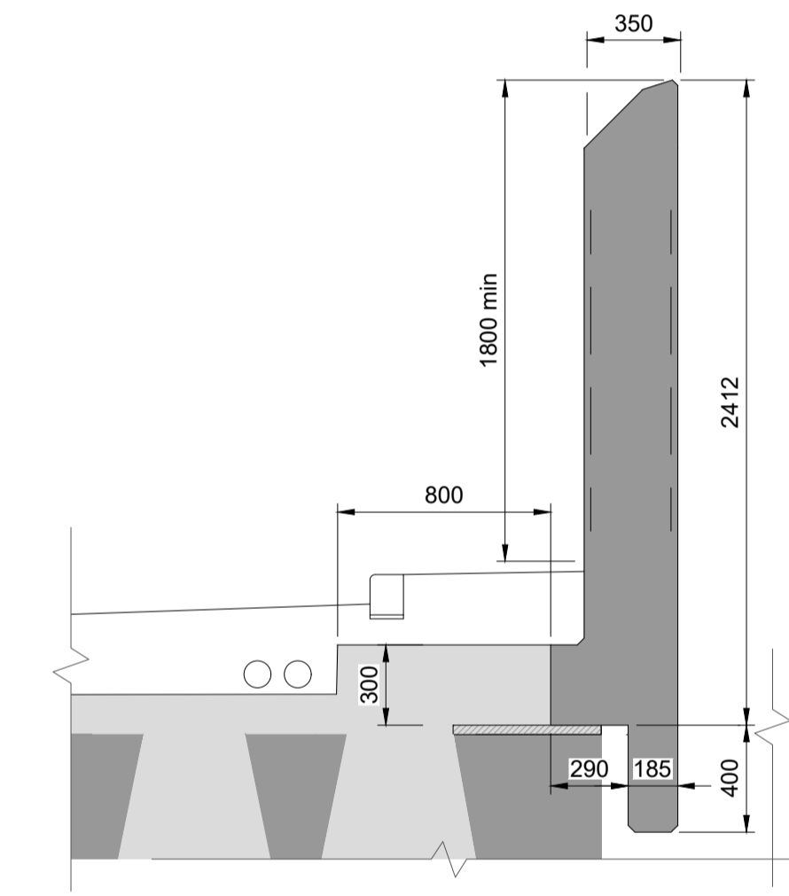
DETAIL 1 Scale 1 : 25 -
