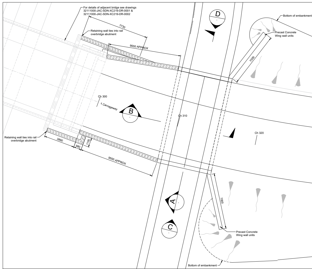
PLAN OF PROPOSED CULVERT (Scale 1:100)
