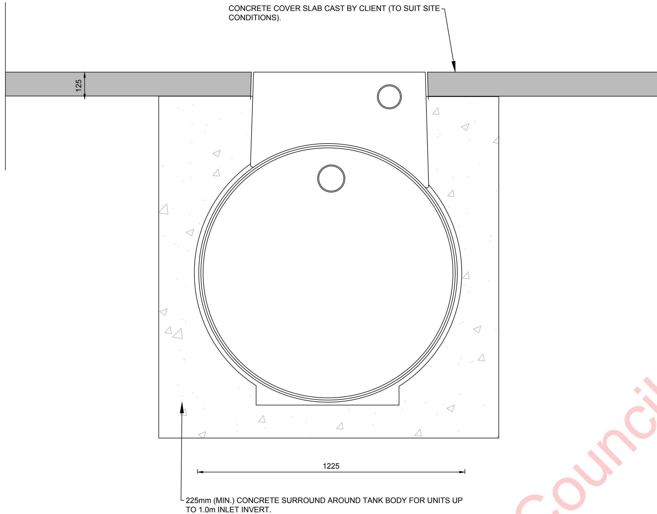
TYPICAL SECTION THROUGH PETROL INTERCEPTOR Scale 1:10
