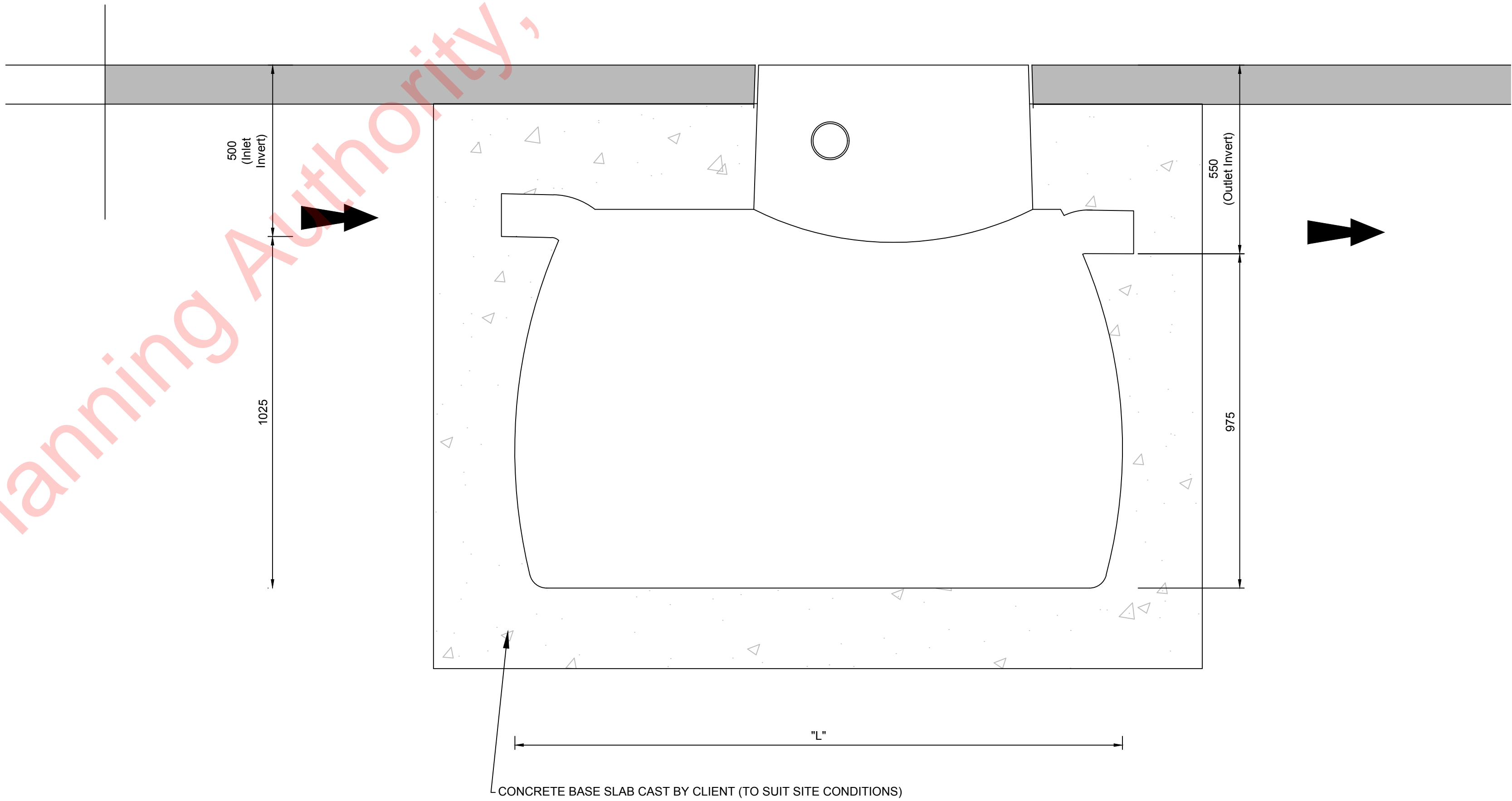
TYPICAL ELEVATION OF PETROL INTERCEPTOR Scale 1:10
