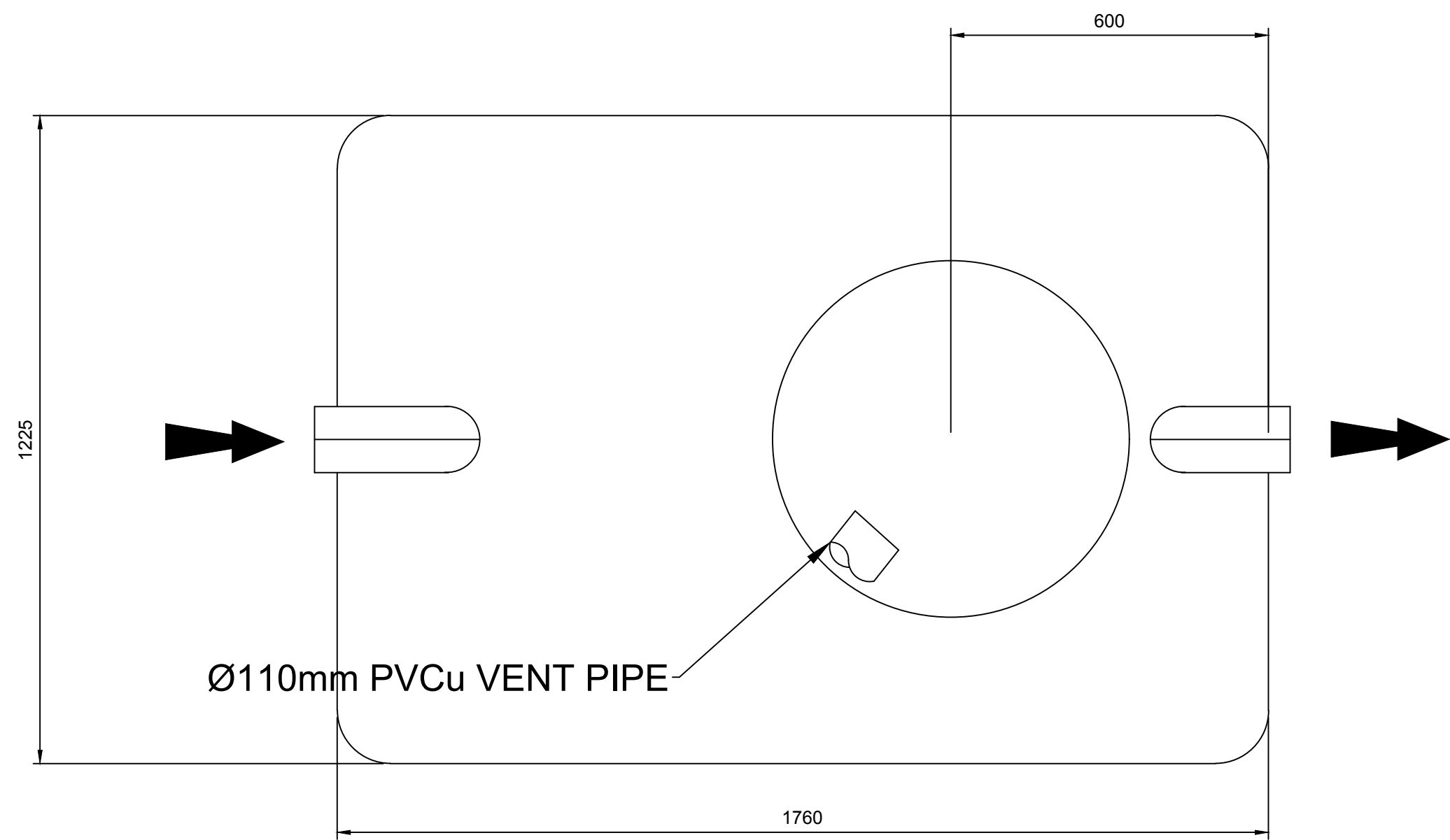
TYPICAL PLAN VIEW OF PETROL INTERCEPTOR Scale 1:10
