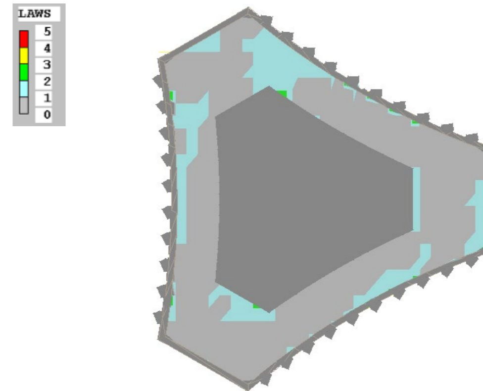
Fig. 3.2.1 - Lawson Criteria at 1.5m above Roof Terrace Level - 2m Balustrade
