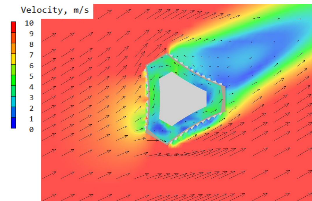
Fig. 2.1.6 Wind Velocity at 90m above Ground Level – 1m Balustrade
