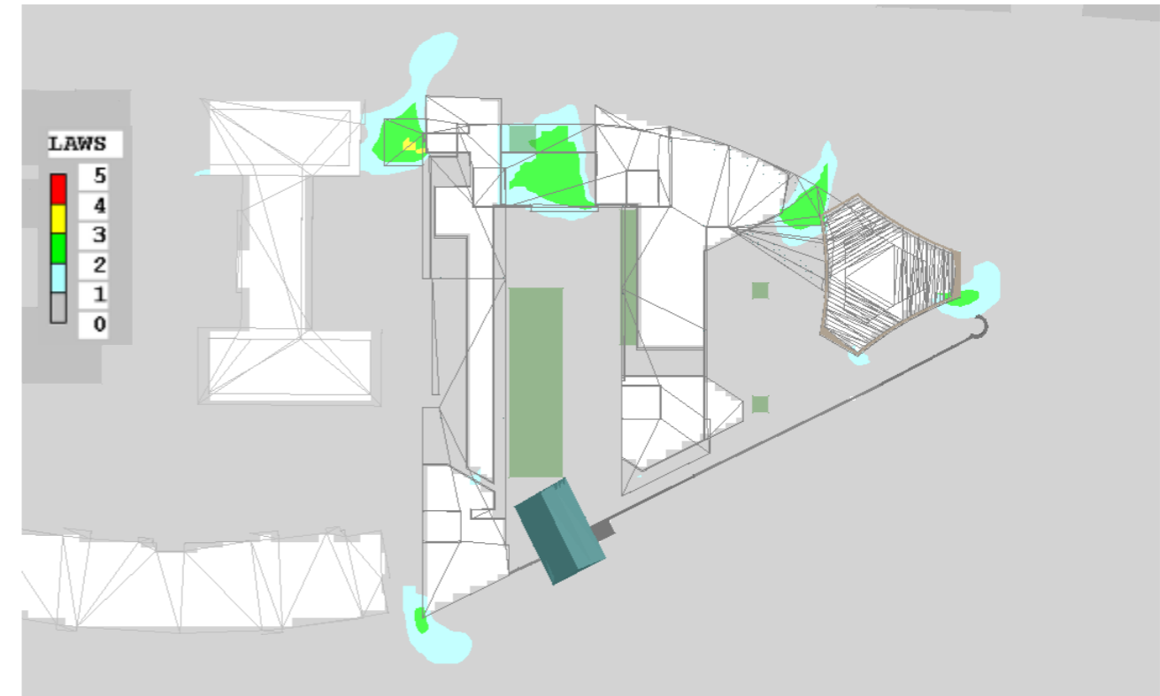
Fig. 4.1.1 - Lawson Criteria at Ground Level
