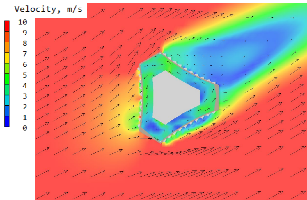
Fig. 2.1.5 Wind Velocity at 90m above Ground Level – No Balustrade
