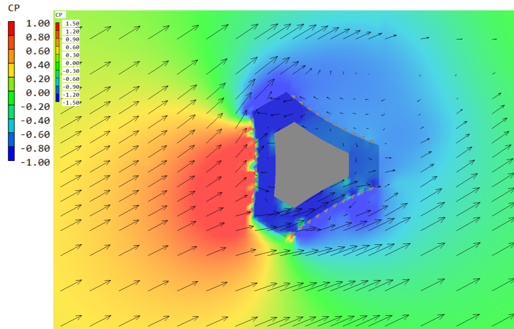
Fig 2.1.3 - Pressure Coefficients at 90m above Ground Level – No Balustrade
