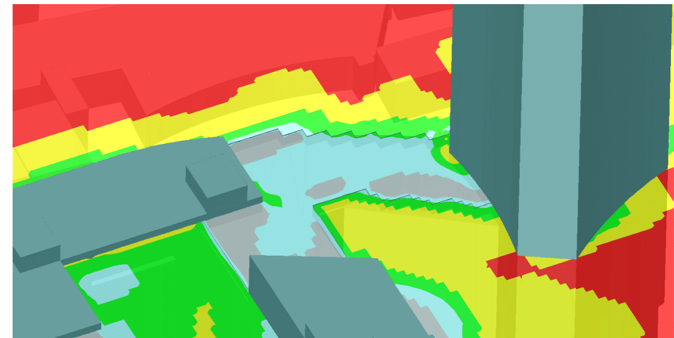
Fig. 4.1.2 - Lawson Criteria at Roof Amenity Level
