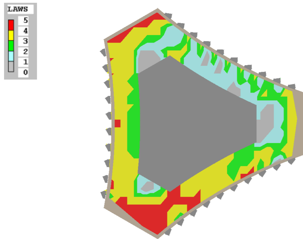
Fig. 3.2.2 - Lawson Criteria at 1.5m above Roof Terrace Level – No Balustrade
