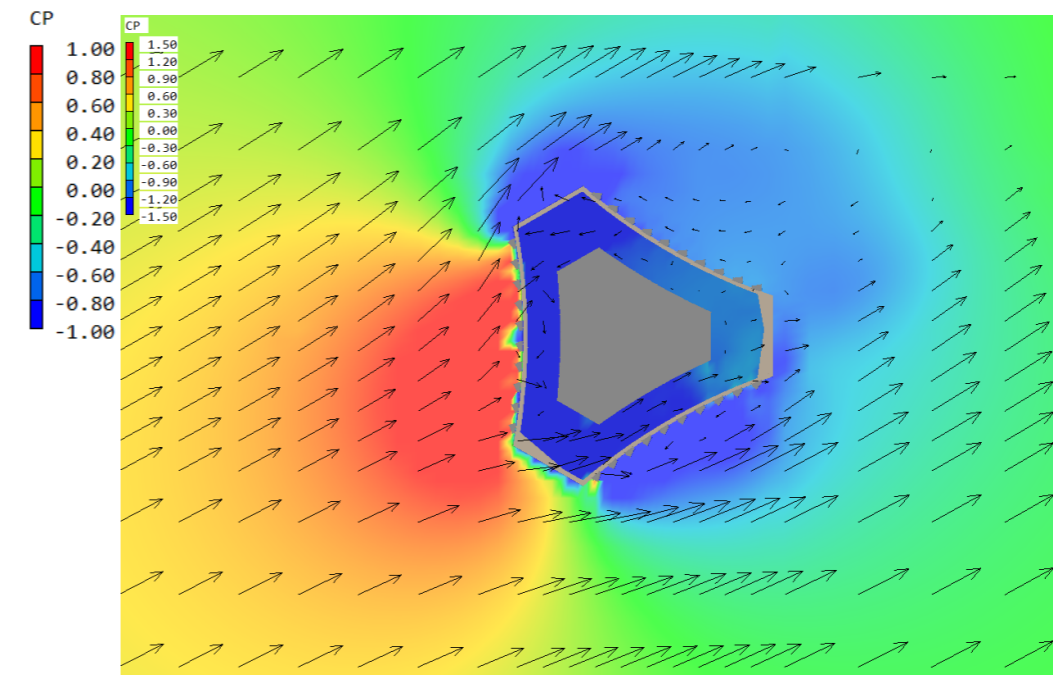
Fig 2.1.4 - Pressure Coefficients at 90m above Ground Level – 1m Balustrade
