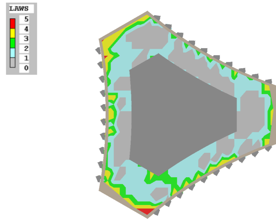
Fig. 3.2.3 - Lawson Criteria at 1.5m above Roof Terrace Level – 1m Balustrade
