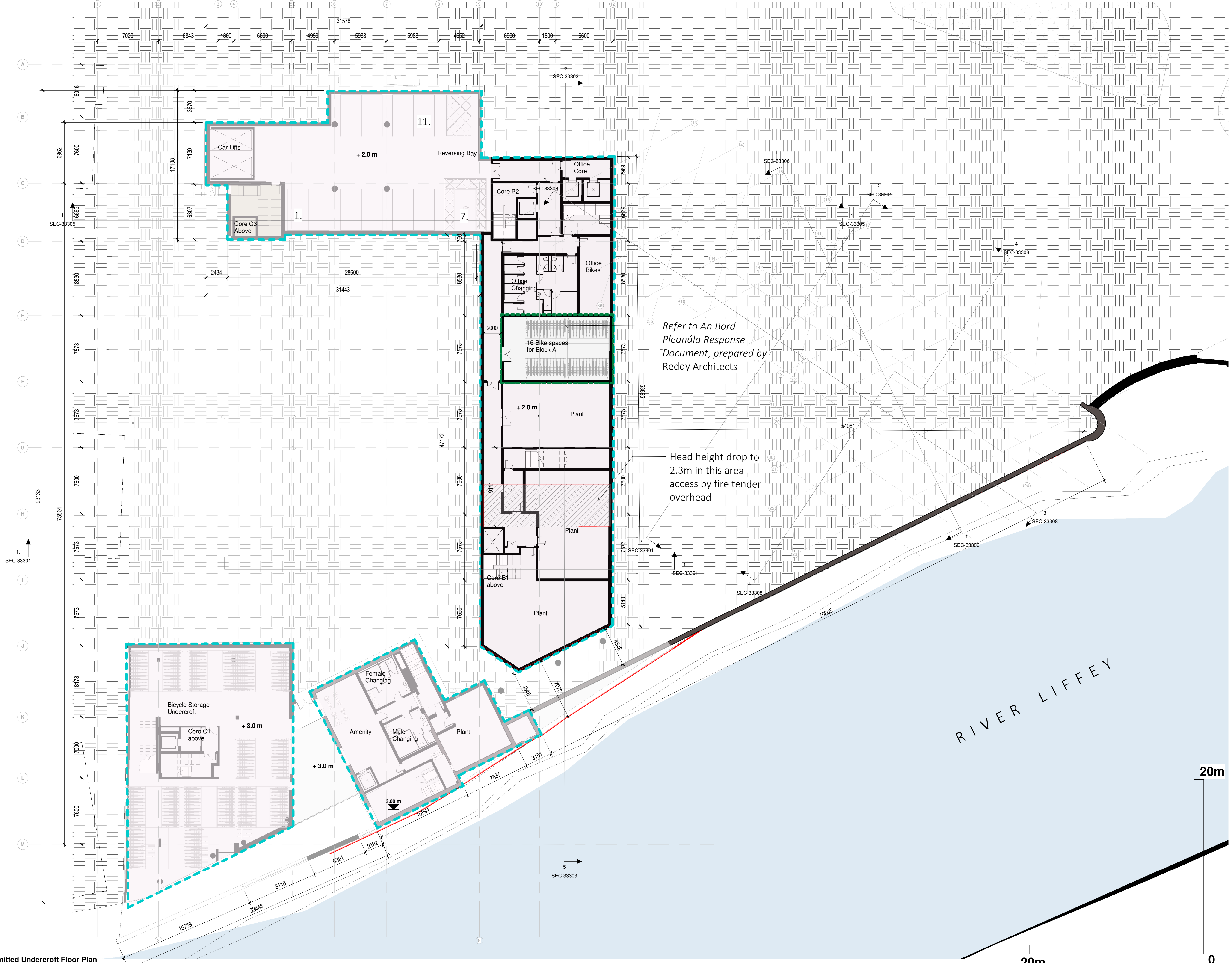
Permitted Undercroft Floor Plan 1:200
