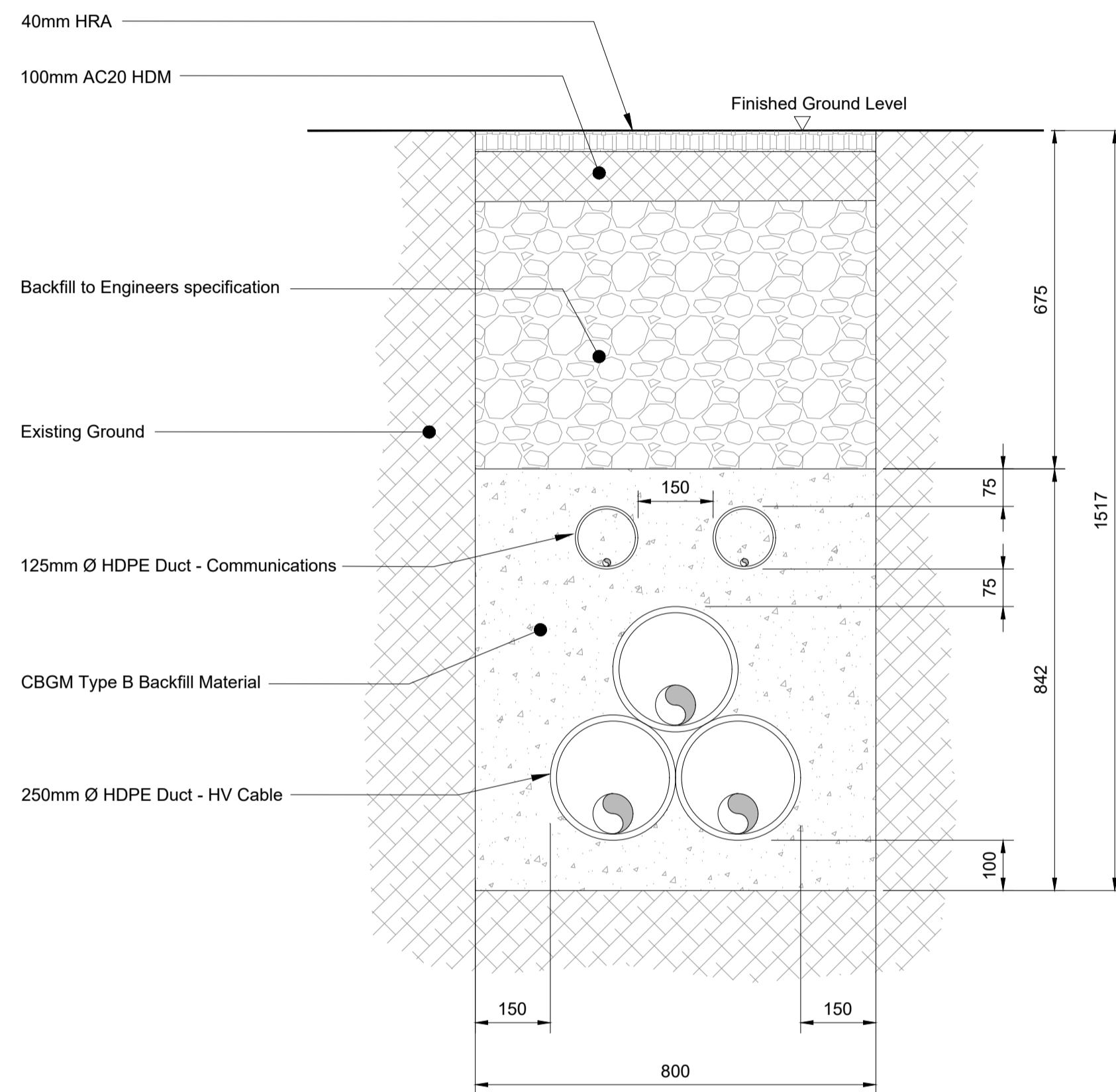
AC Cable - Typical Section 1:10
