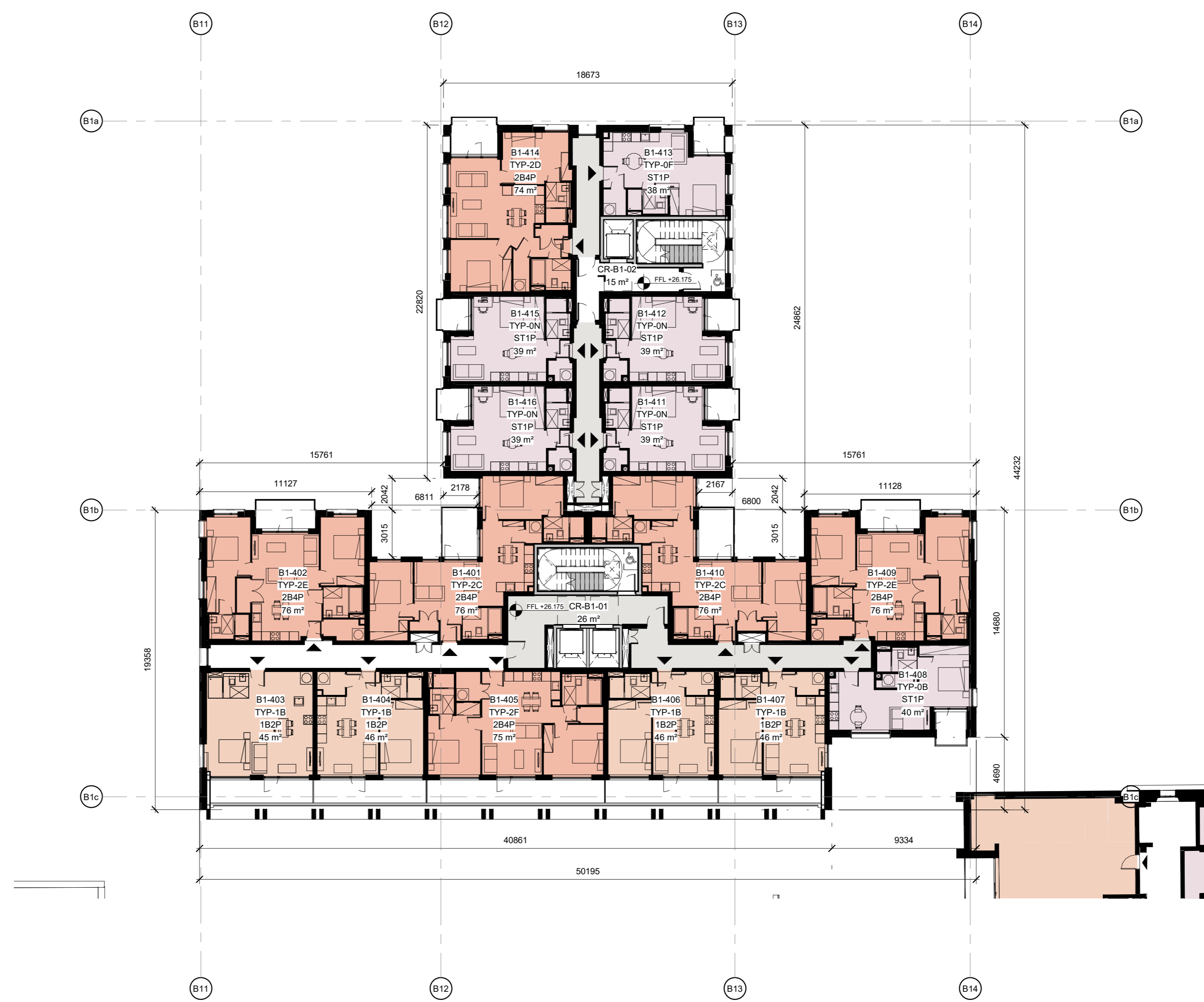
2 BLOCK B1-LEVEL 04 1 : 200
