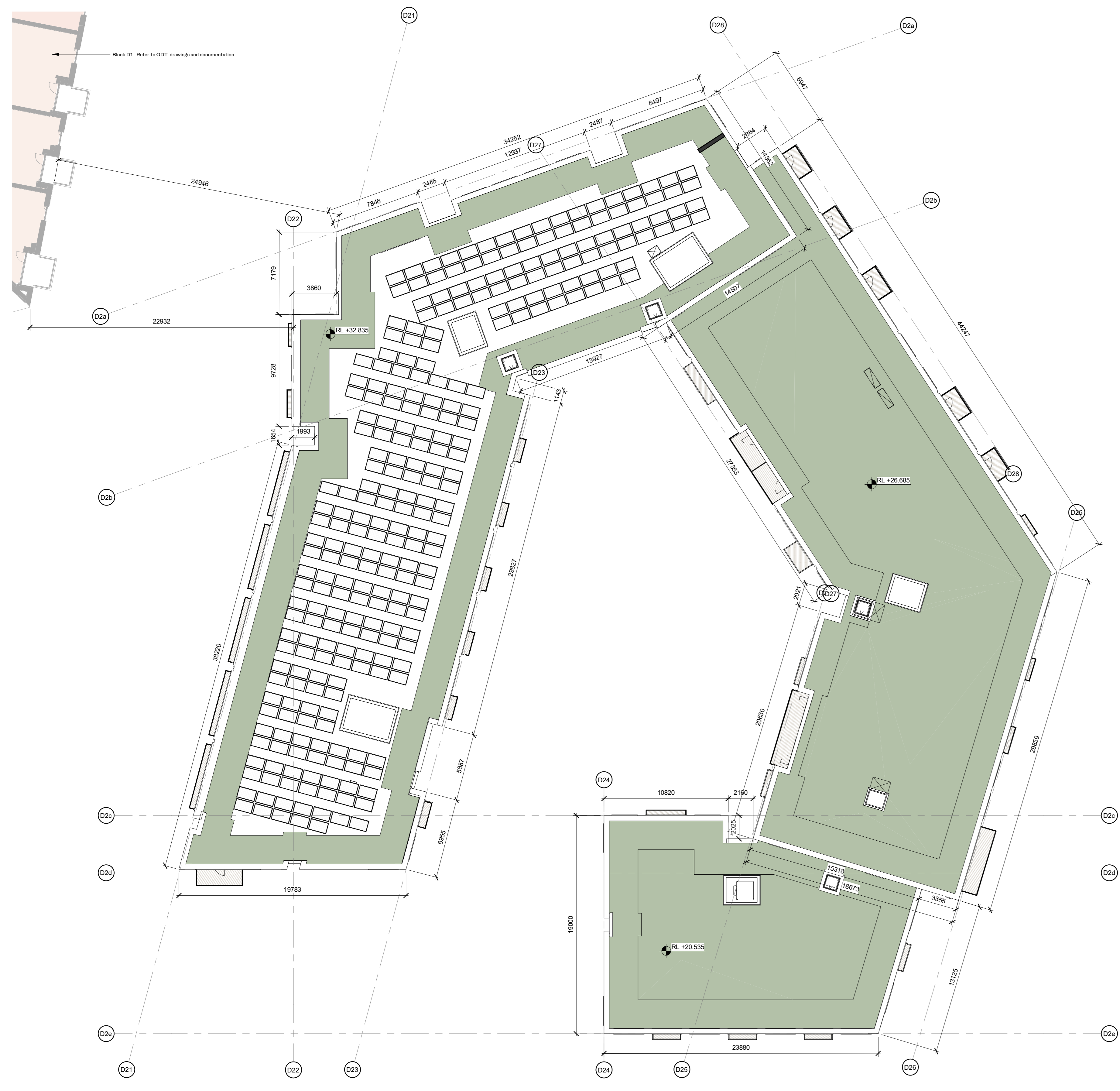
1 BLOCK D2-LEVEL 08 1 : 200
