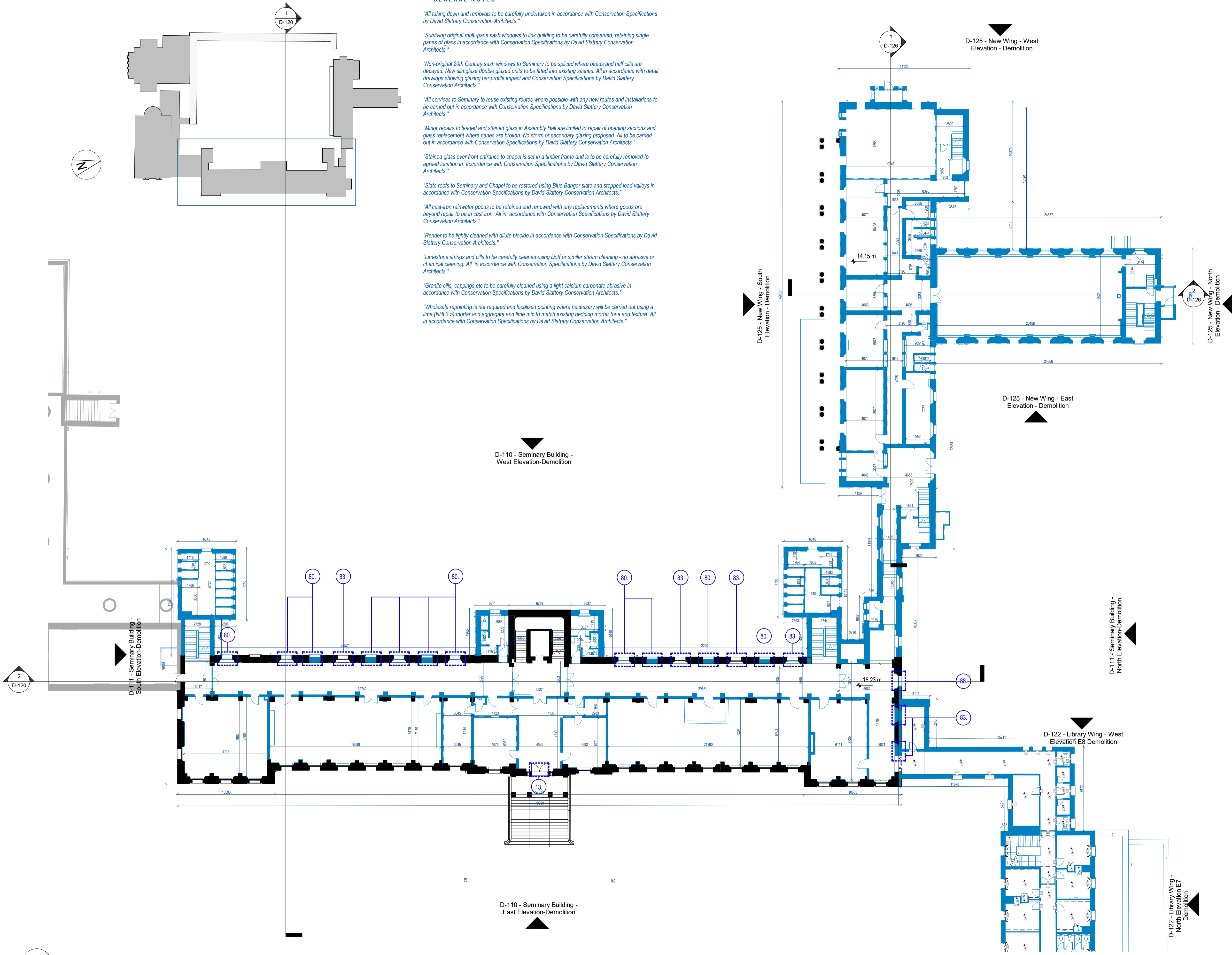
1 Seminary Building - First Floor Demolition Plan Scale - 1 : 200
