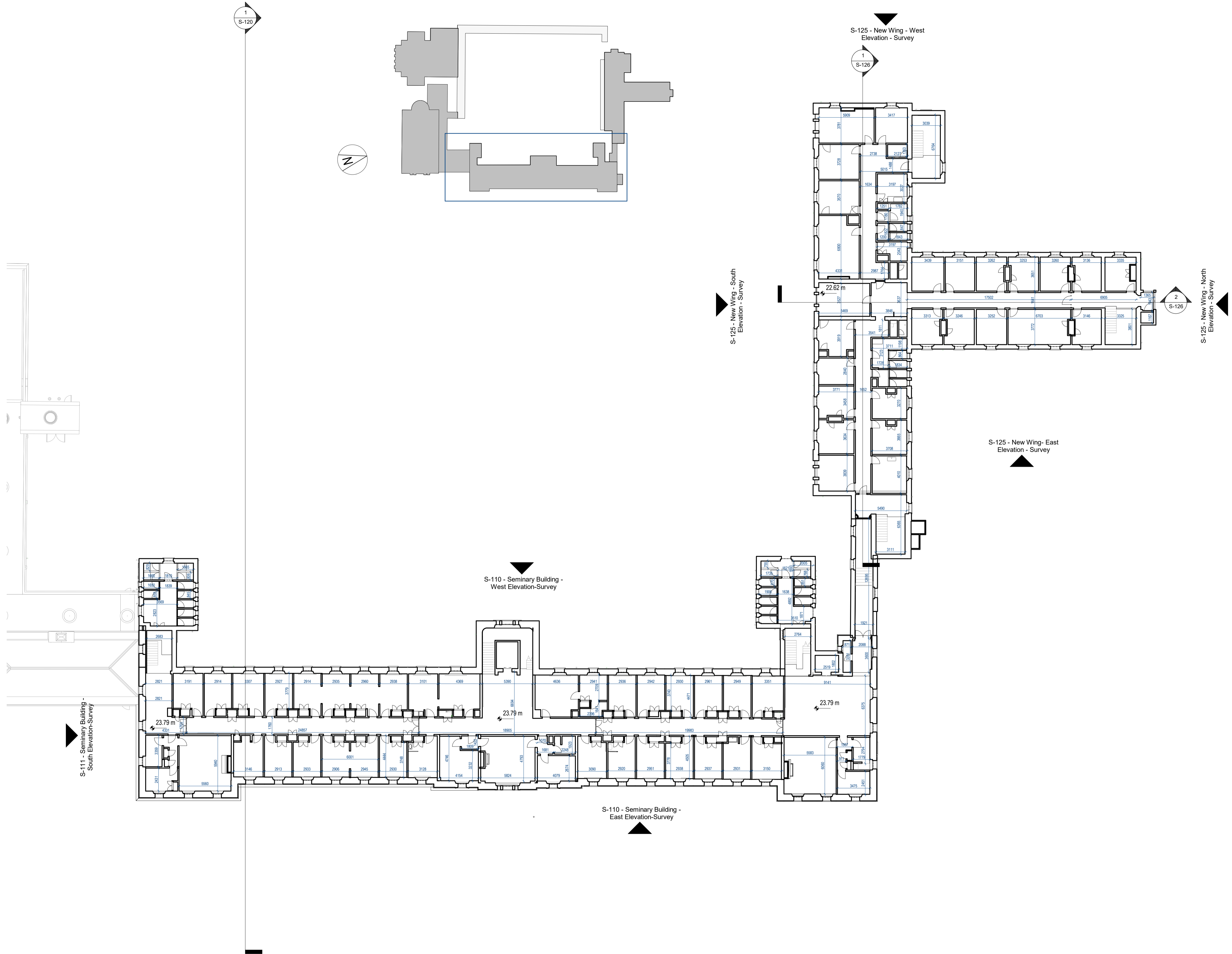
1 Seminary Building - Third Floor Plan-Survey Scale - 1:200
