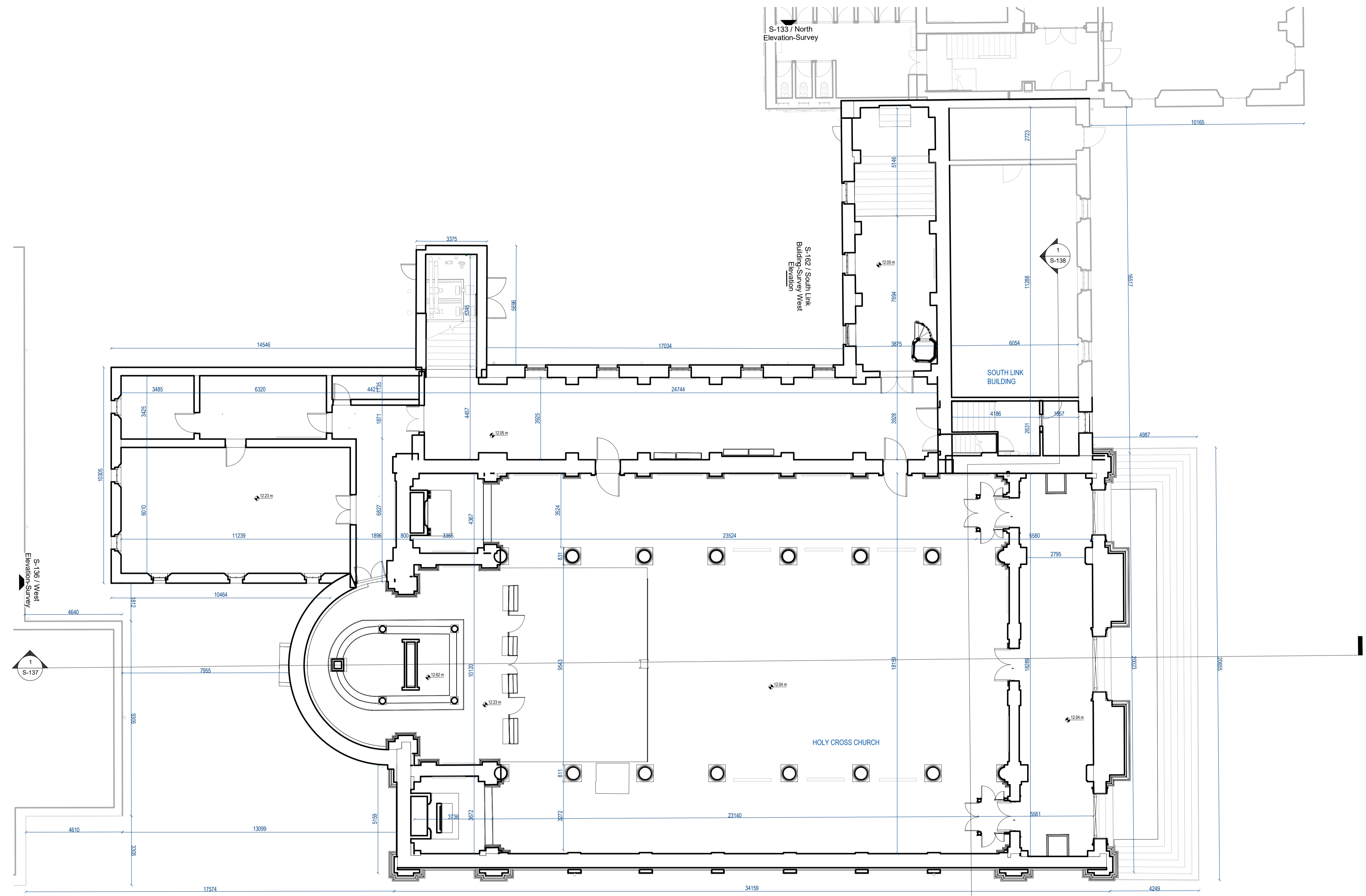
1 08 Floor-Survey Scale - 1:100
