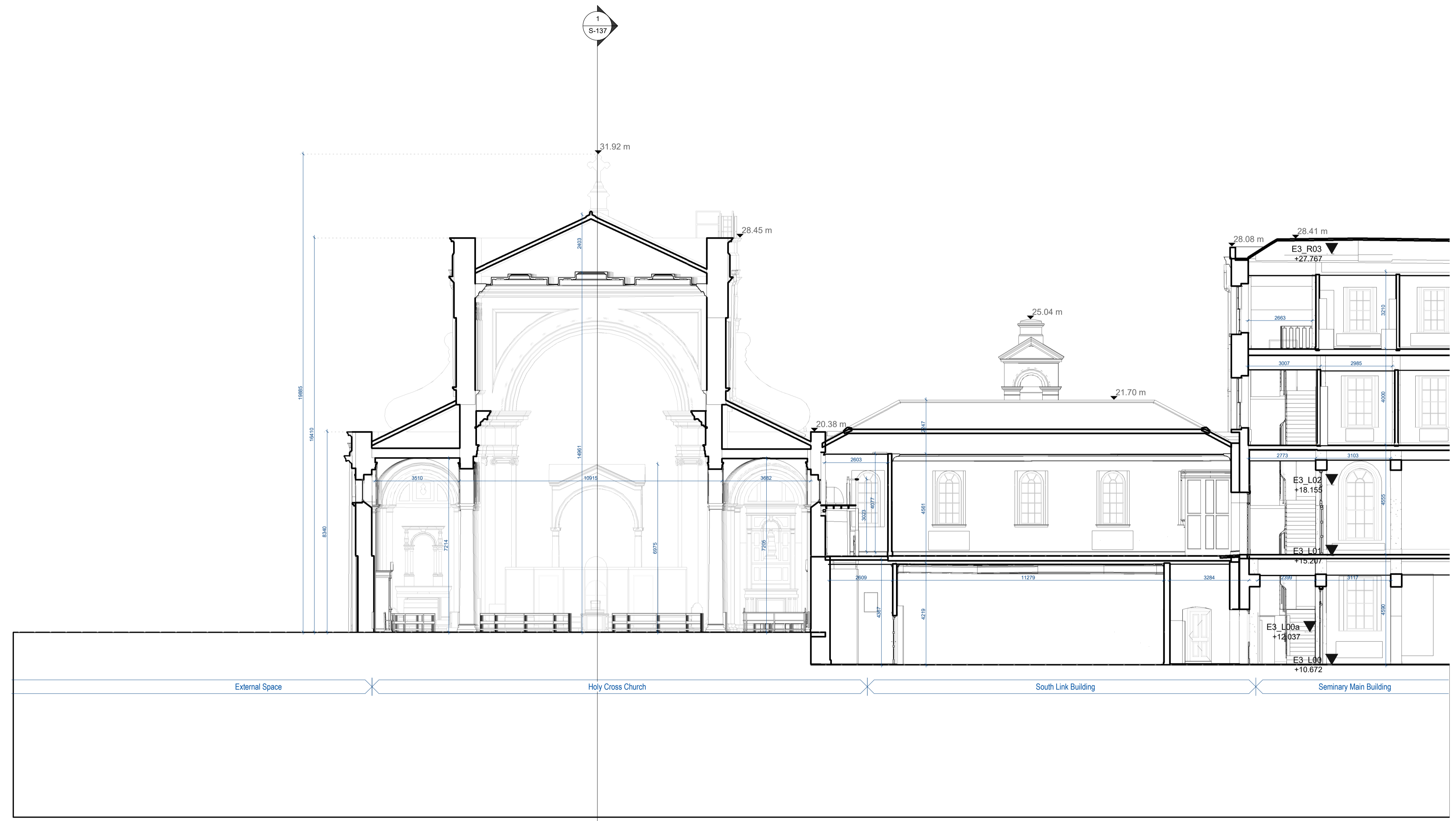
1 Section-CC-Survey Scale - 1:100
