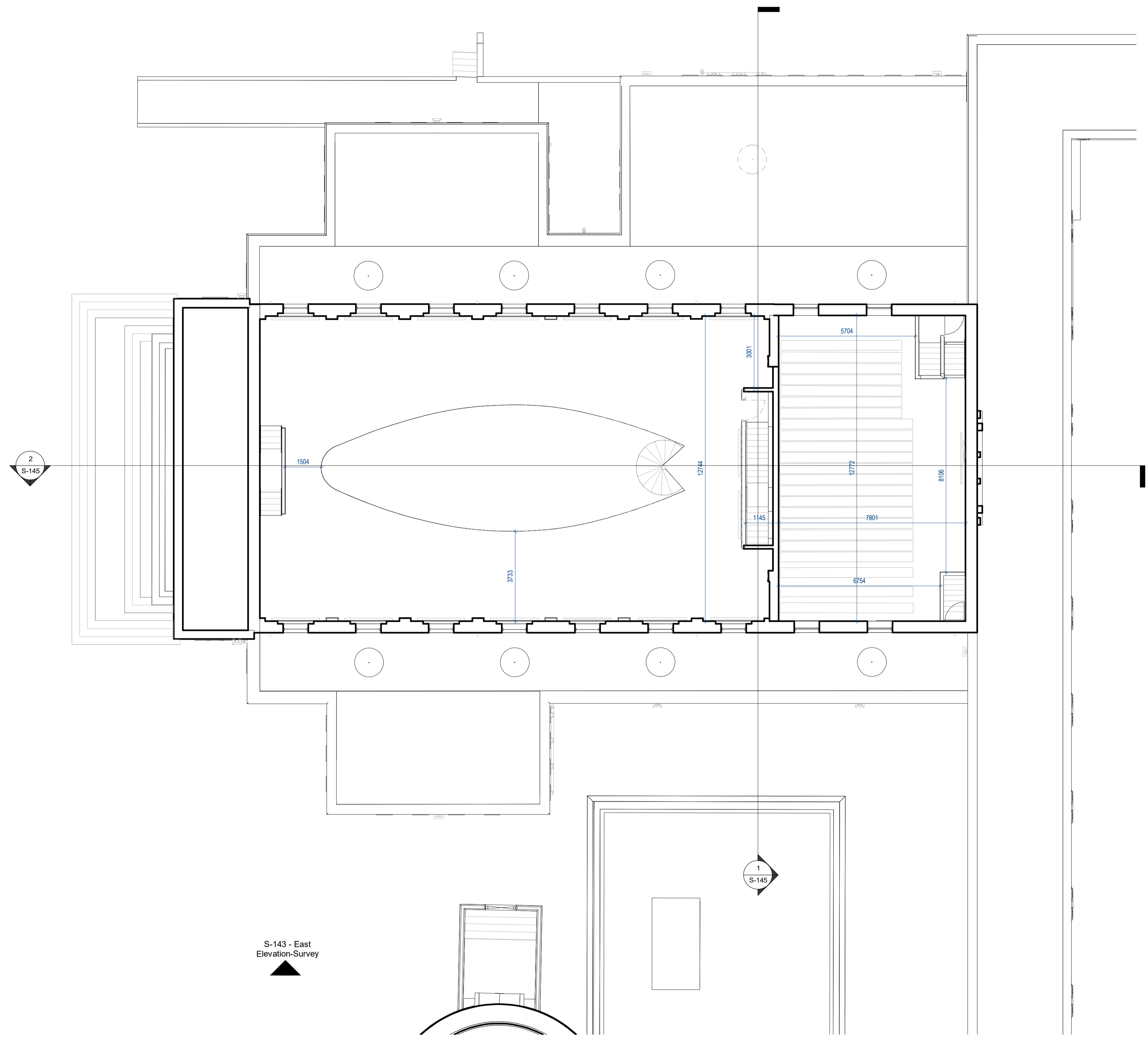
1 First Floor-Survey Scale - 1:100
