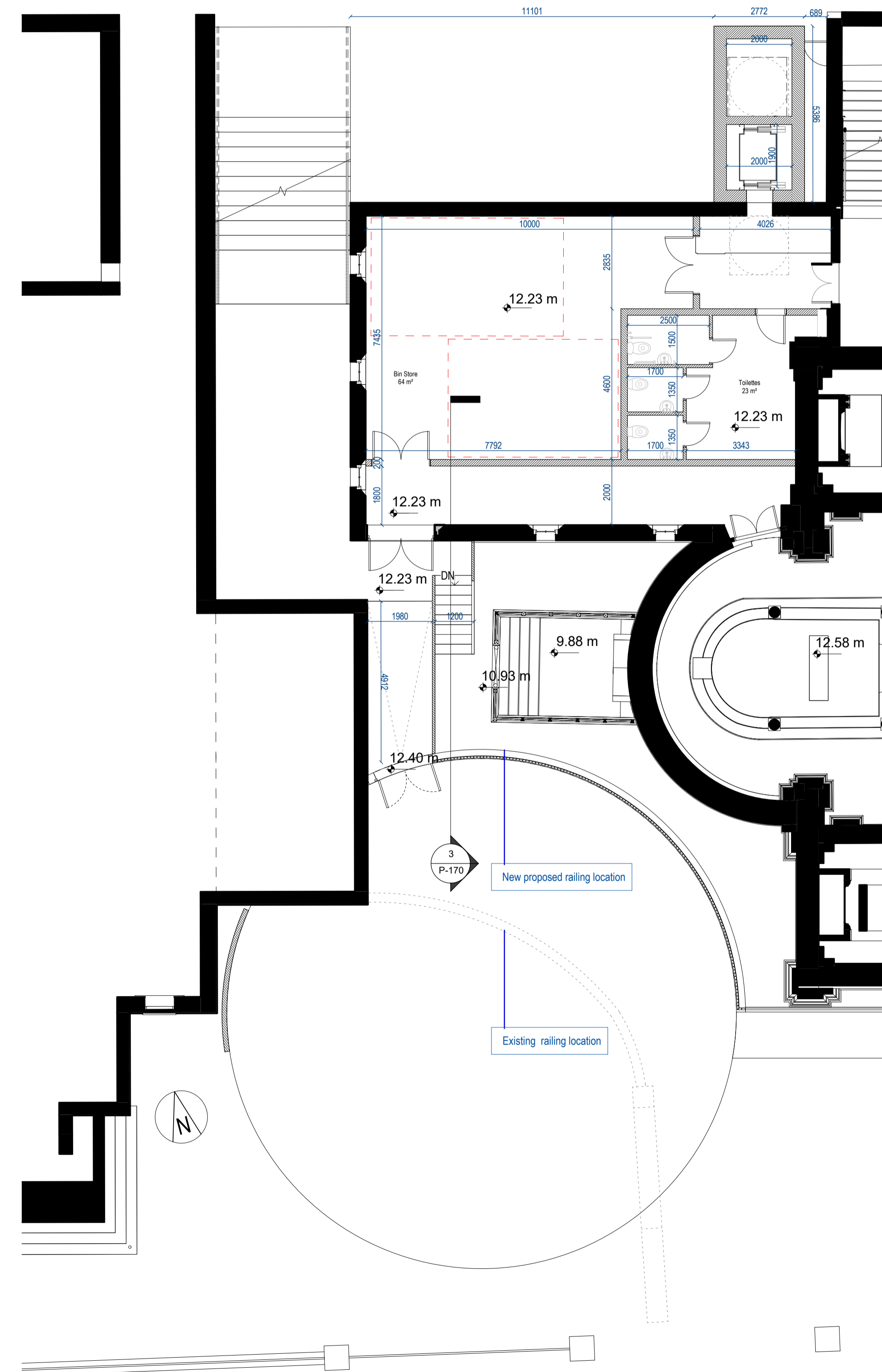
1 Church - Turning Circle Scale - 1:100
