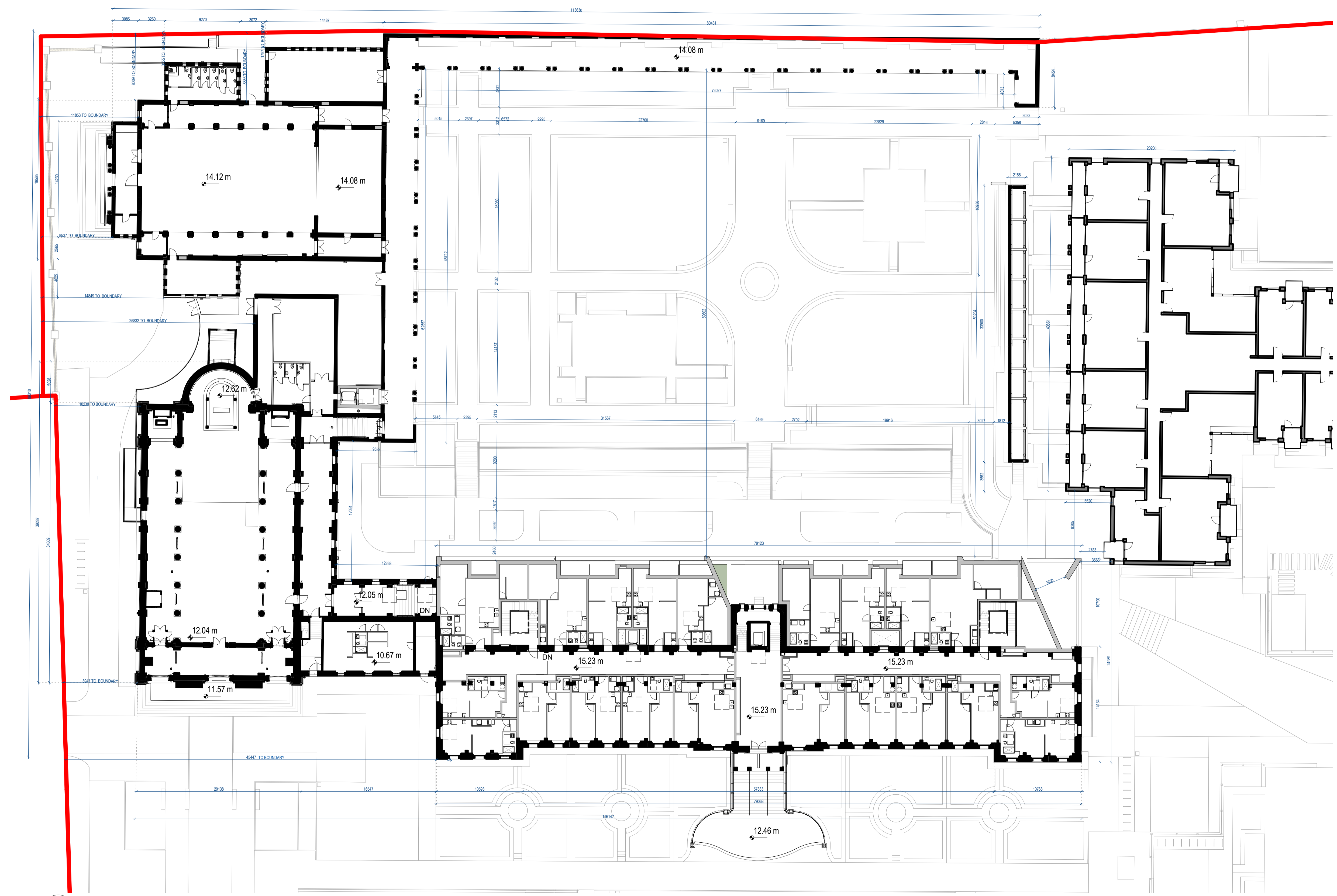
1 Site Layout Plan - Proposed Scale - 1: 250
