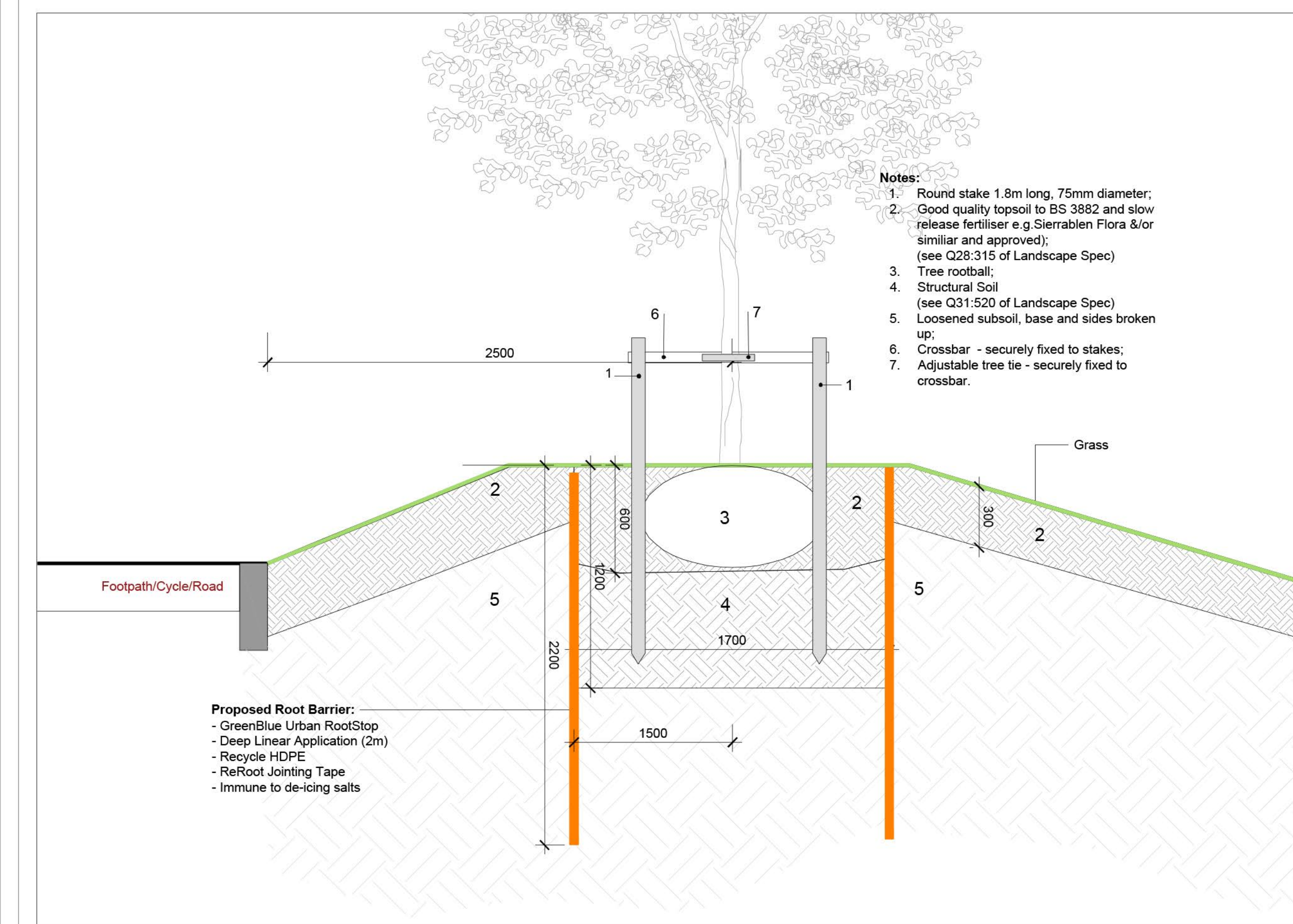
Typical Detail of Root Protection Barrier 1:20
