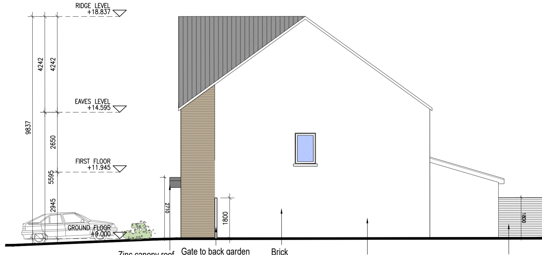
Type A5- Side Elevation - Maynetown 1:100@A1 3 BED HOUSE
