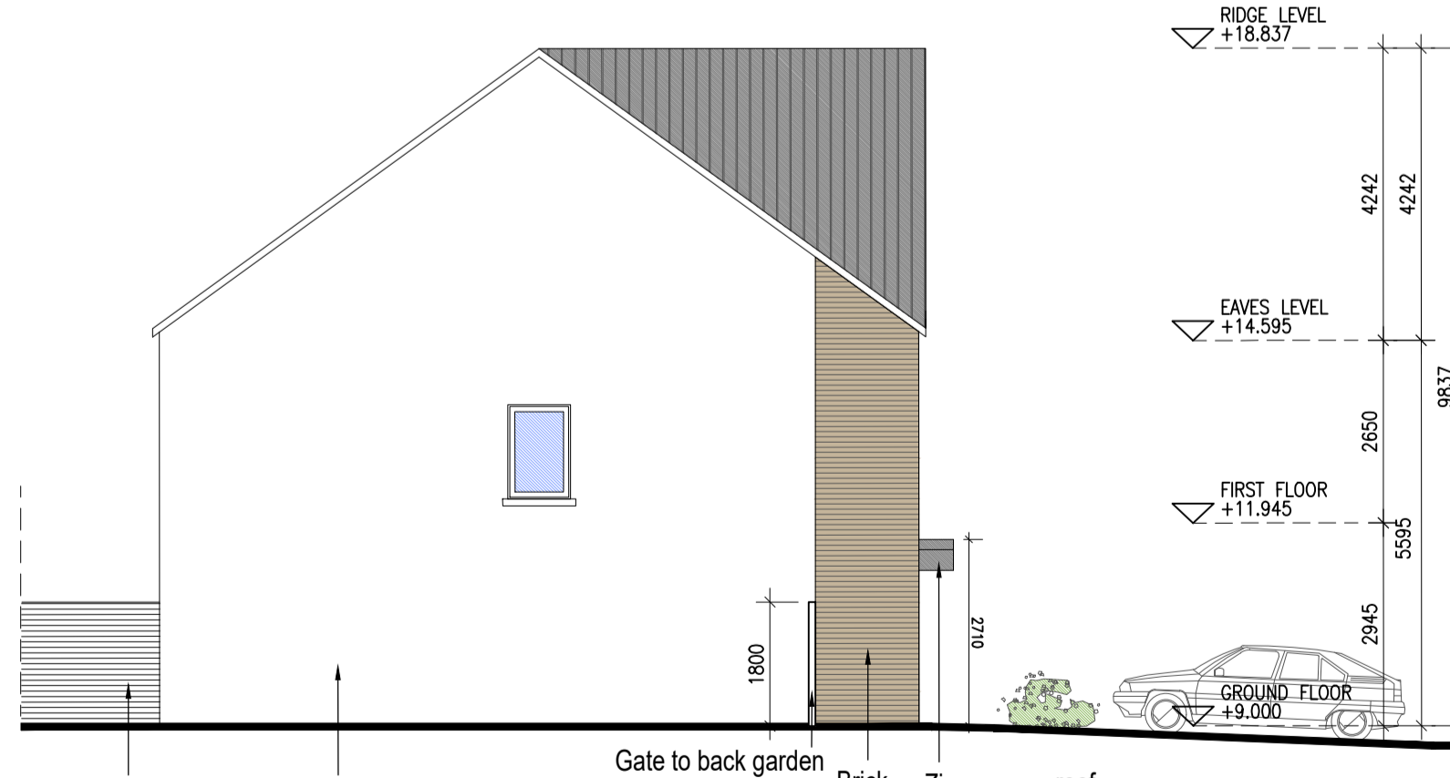
Type B3 - Side Elevation - Maynetown 1:100@A1 3 BED HOUSE
