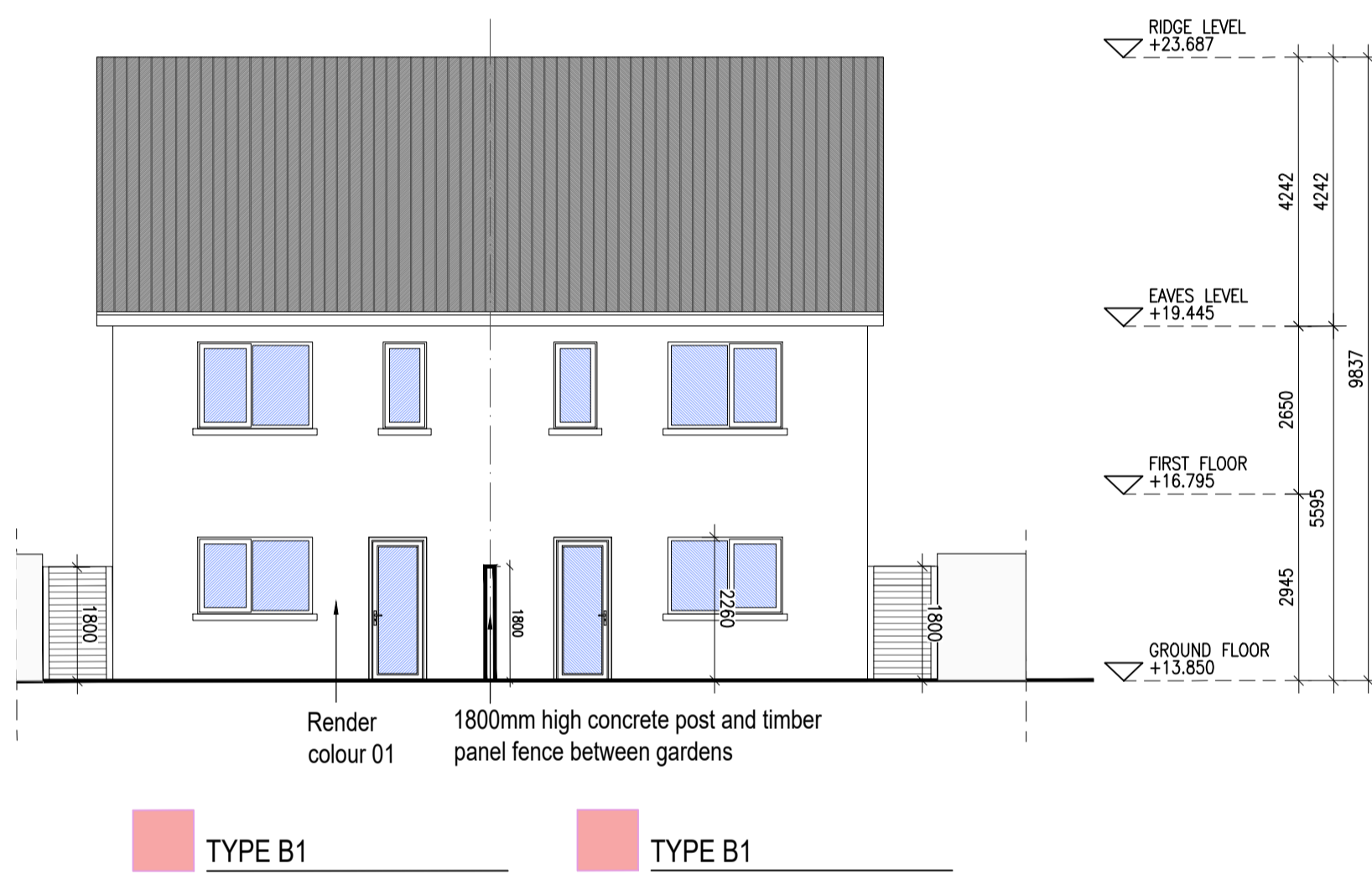
02 Type B1 - Rear Elevations 1:100@A1 3 BED HOUSE
