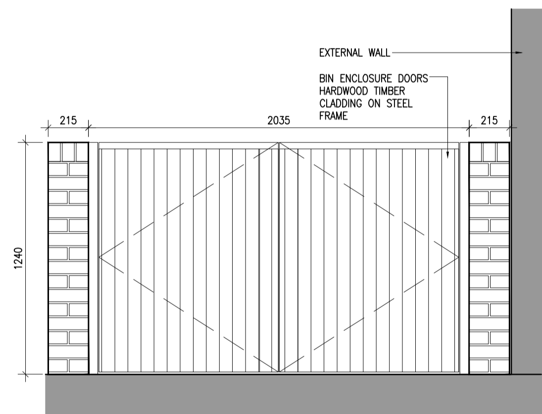
2 Bin store Type 3 Side Elevation P203 Scale 1:20
