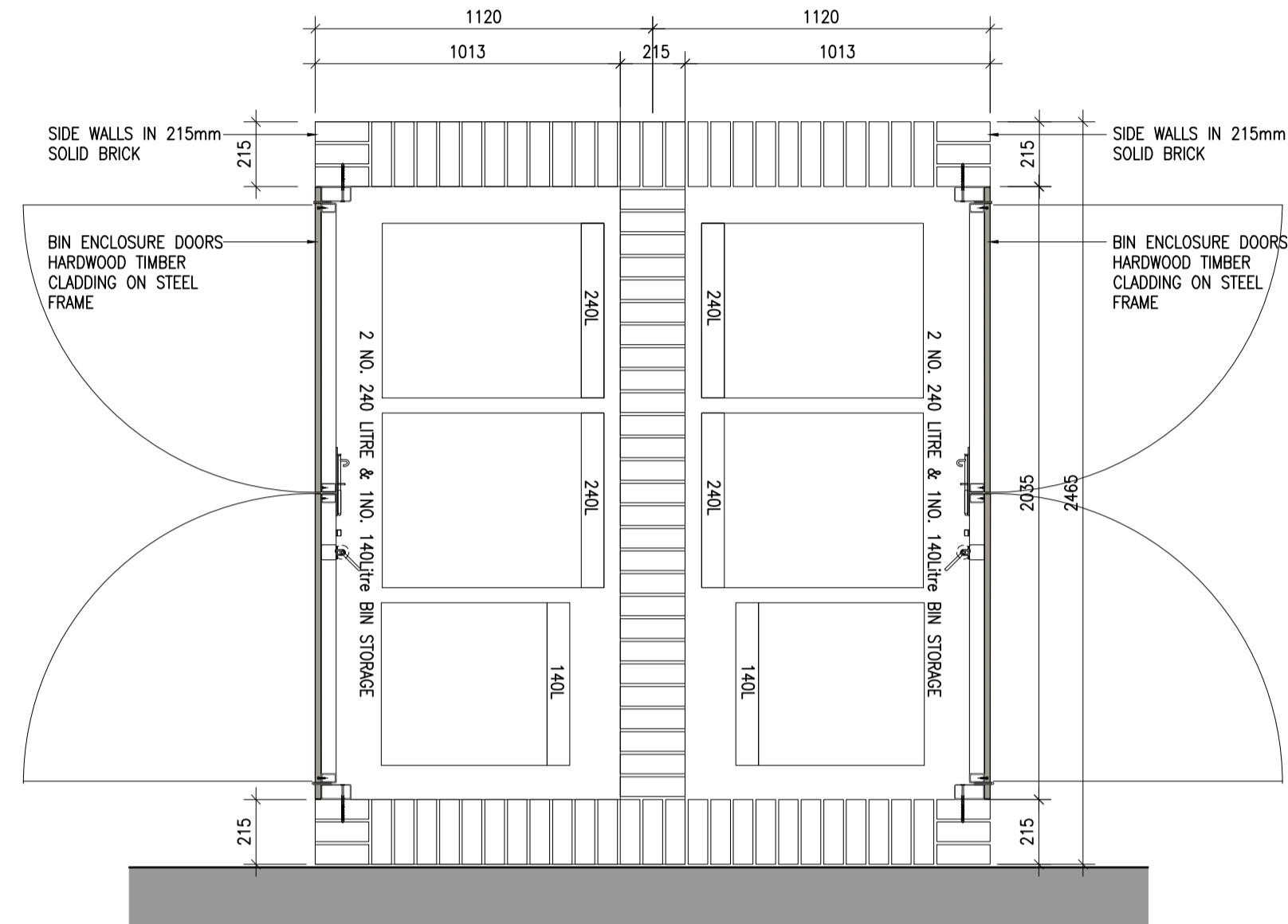
1 Bin store Type 3 Plan P203 Scale 1:20
