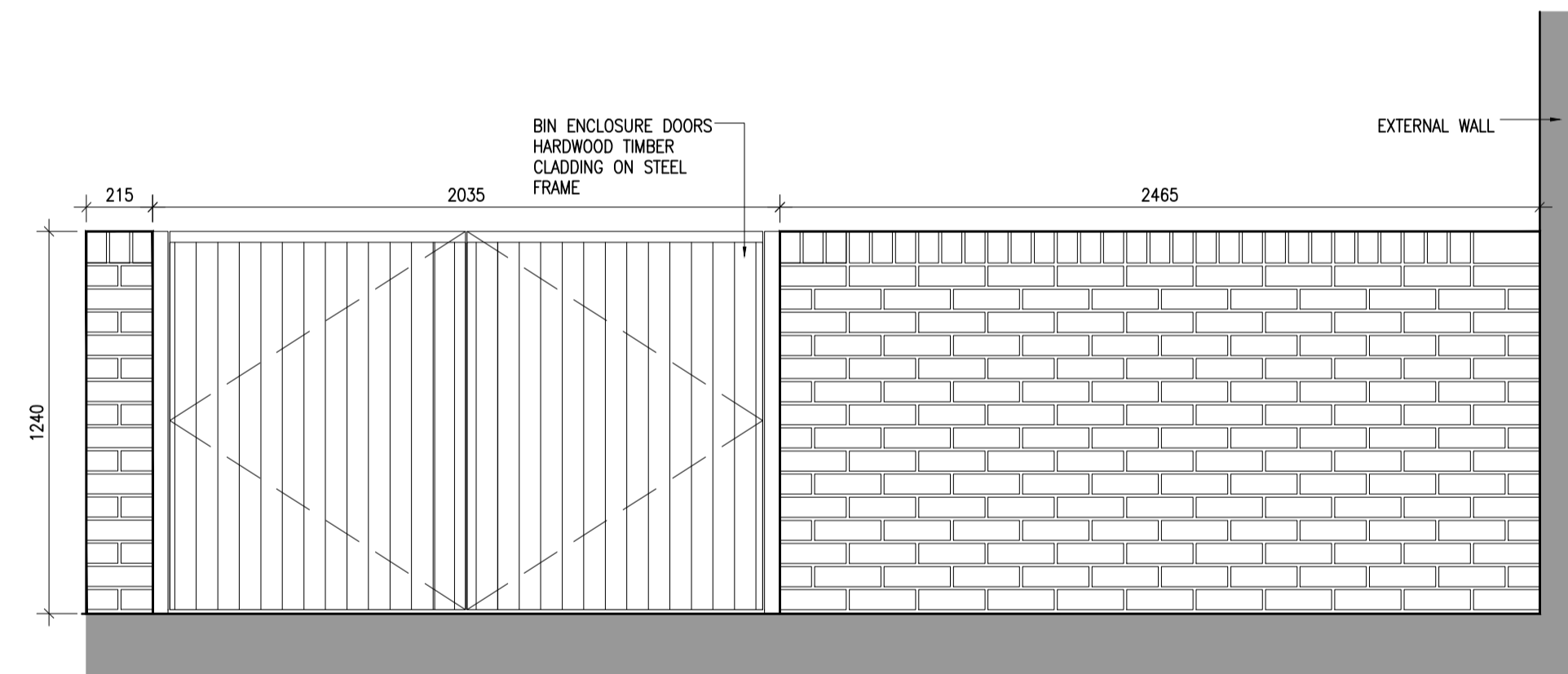
2 Bin store Type 4 Front Elevation P203 Scale 1:20
