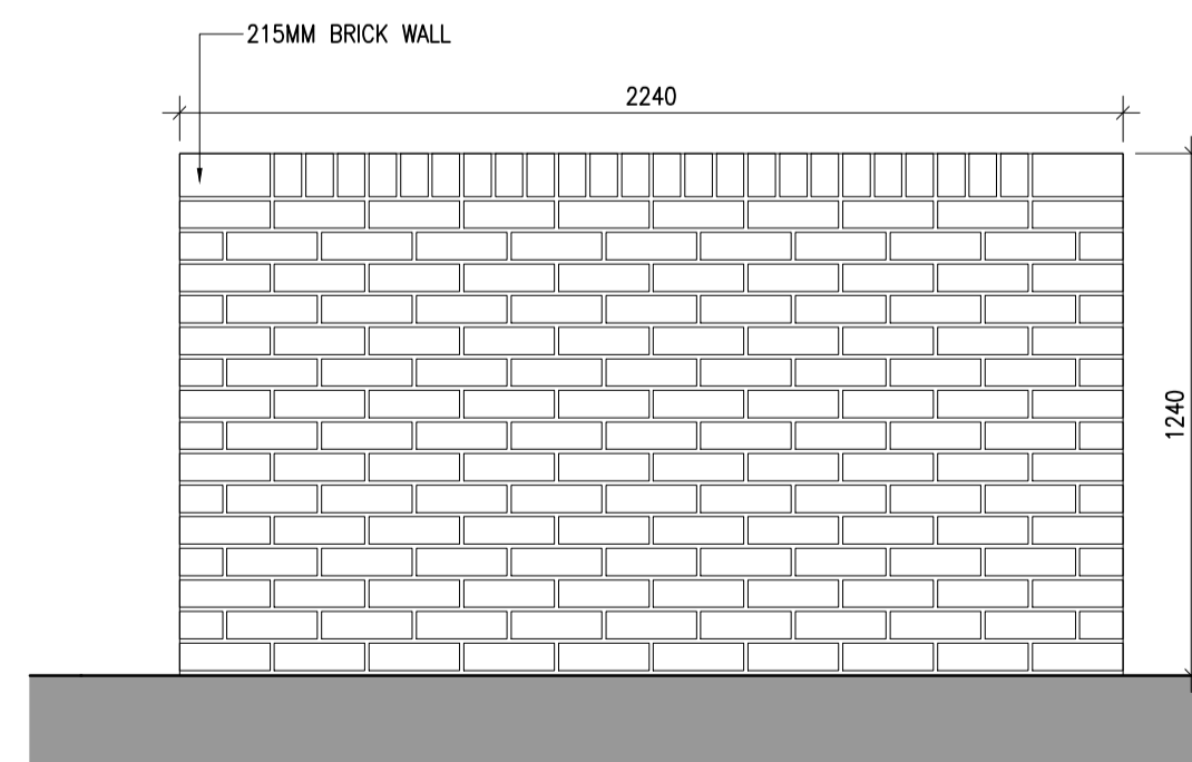
3 Bin store Type 3 Front P203 Scale 1:20
