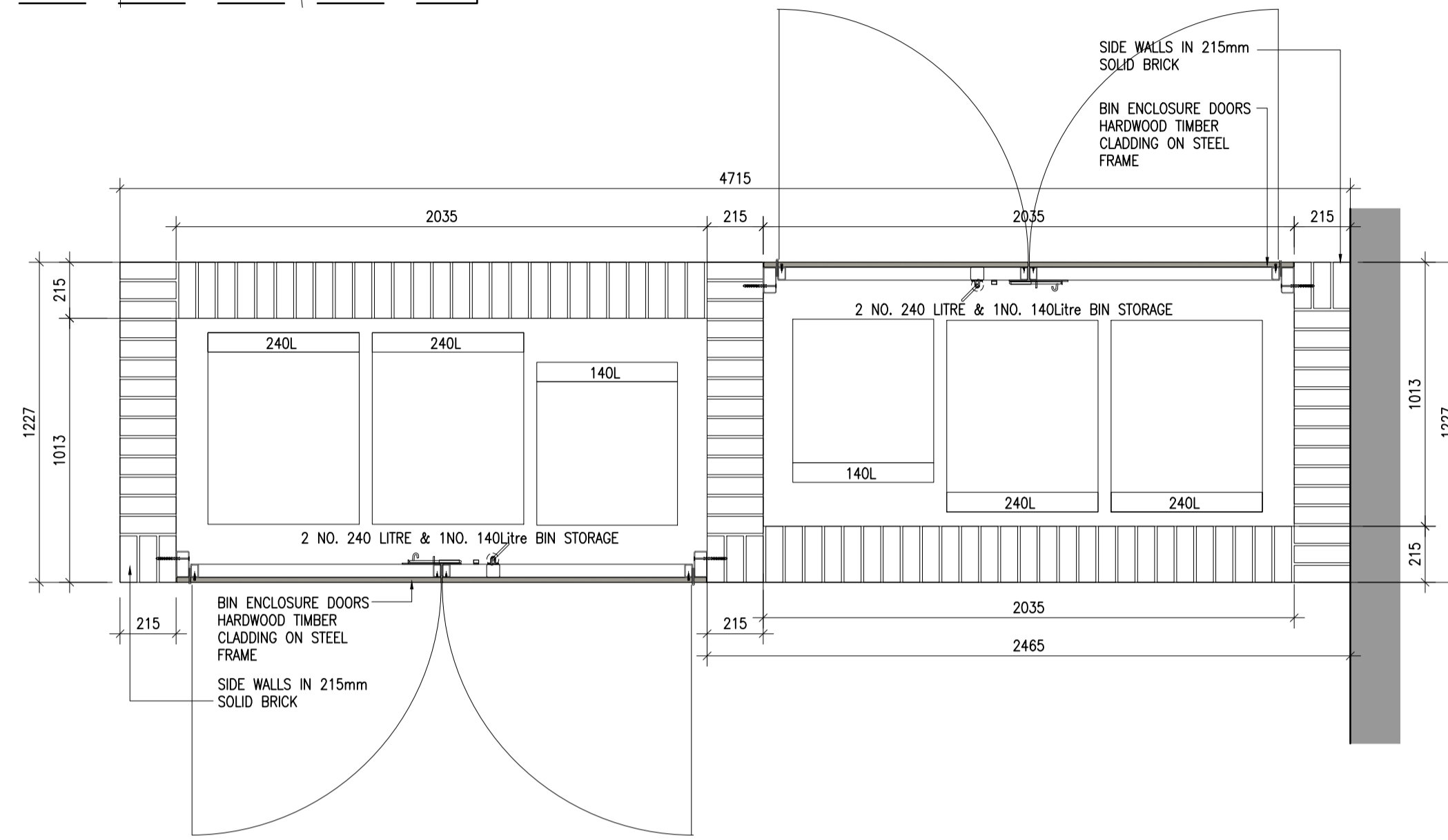
1 Bin store Type 4 Plan P203 Scale 1:20
