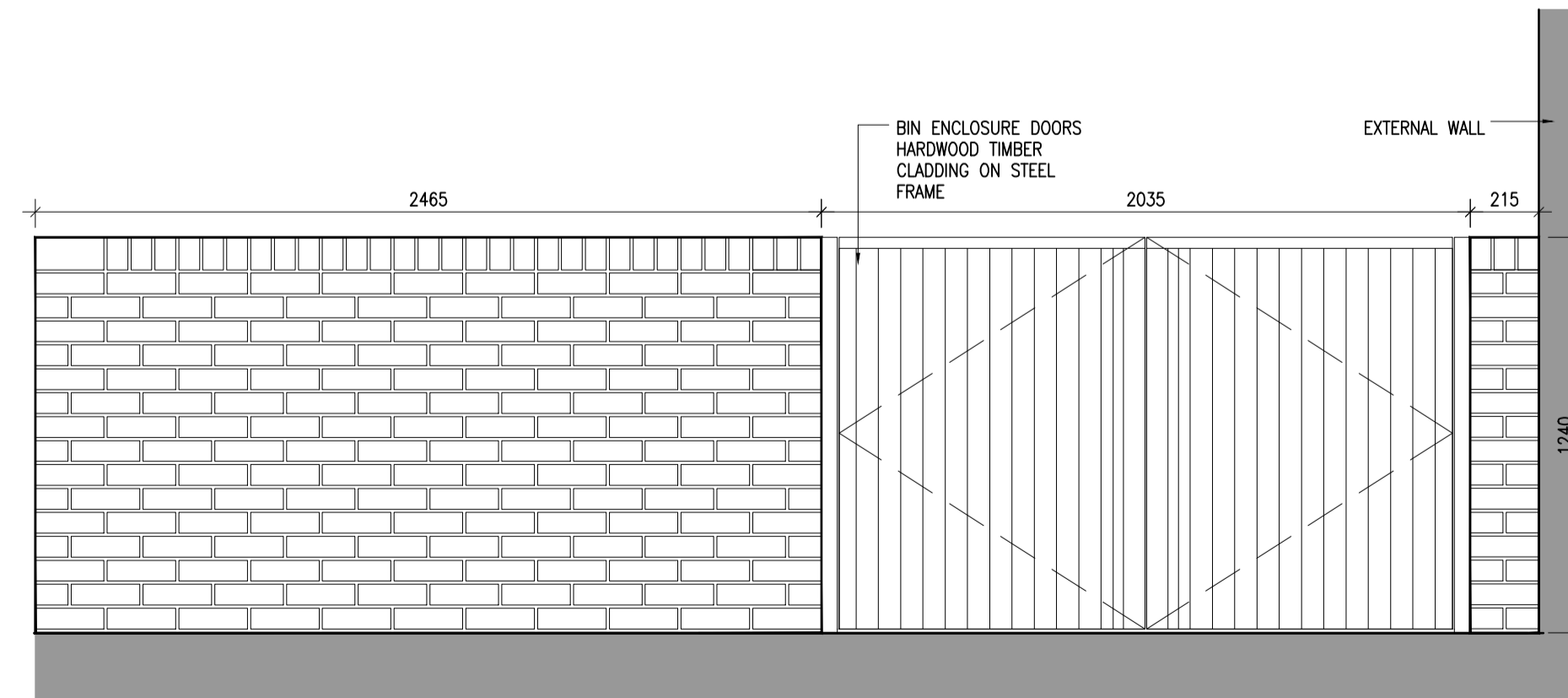
3 Bin store Type 4 Rear Elevation P203 Scale 1:20
