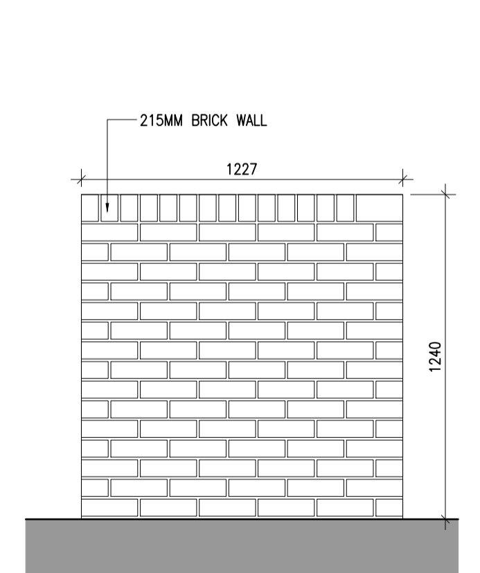
4 Bin store Type 4 Side Elevation P203 Scale 1:20
