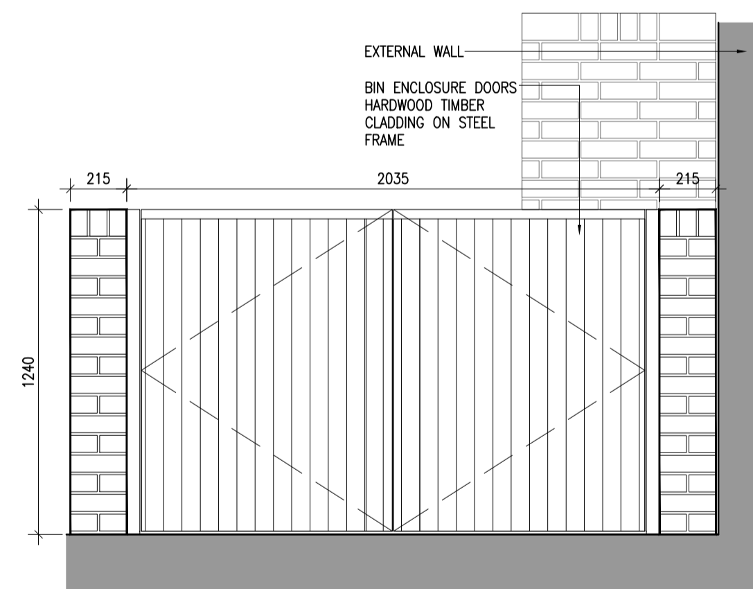
3 Bin store Type 7 Rear Elevation P205 Scale 1:20
