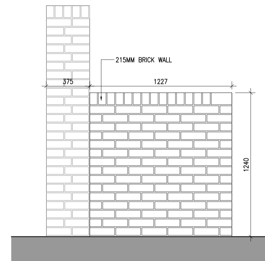
4 Bin store Type 7 Side Elevation P205 Scale 1:20
