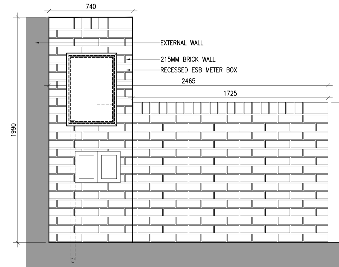
2 Bin store Type 7 Front Elevation P205 Scale 1:20
