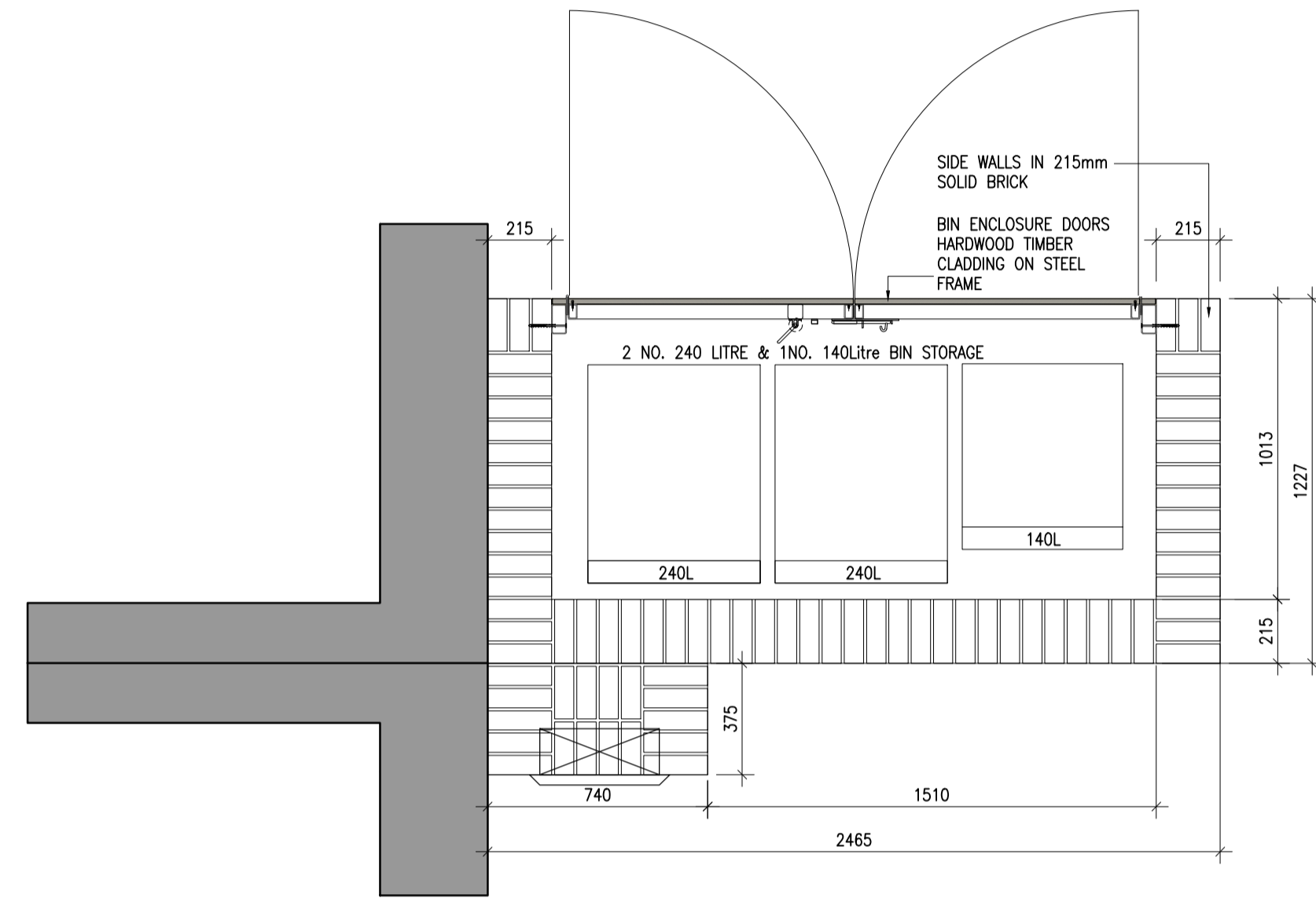
1 Bin store Type 7 Plan P205 Scale 1:20
