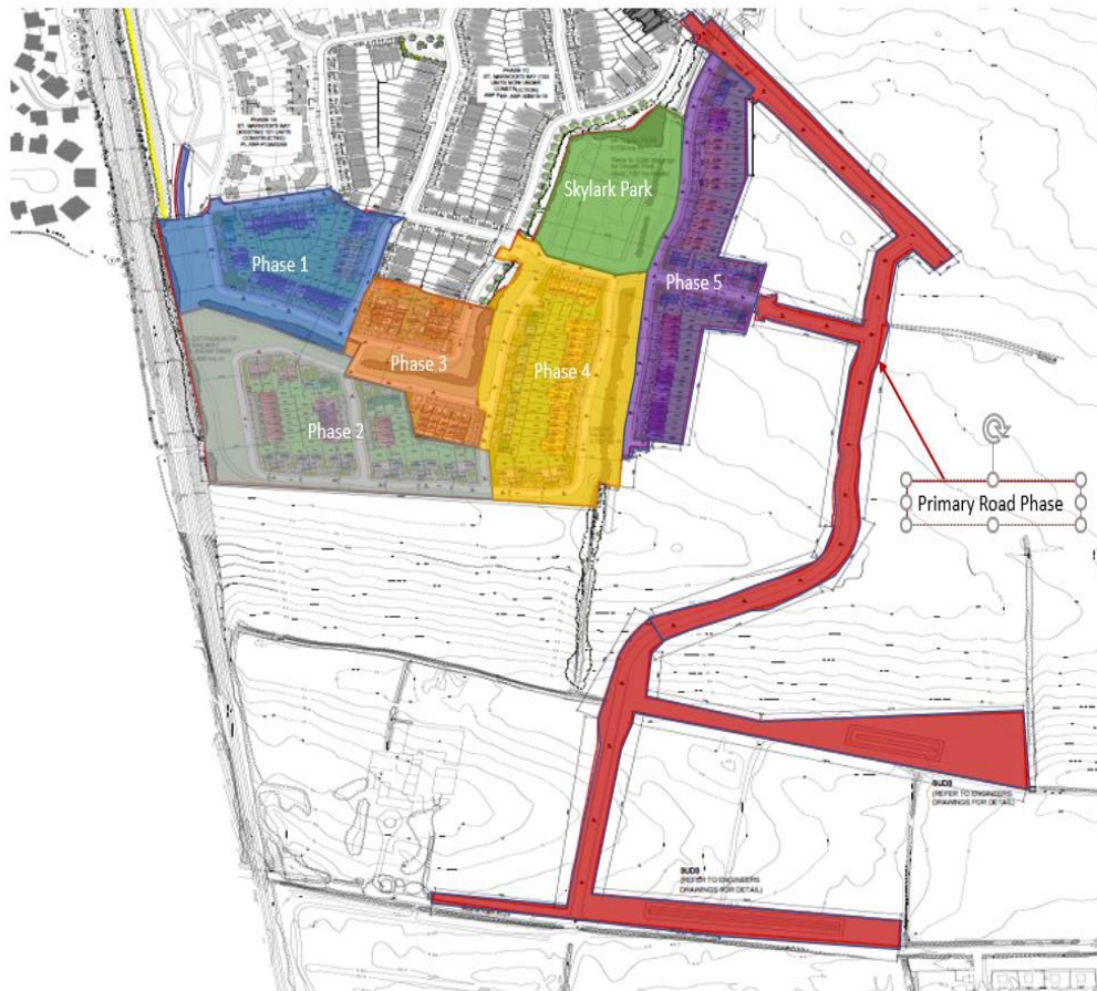
Figure 1.0: Indicative Site Construction Phasing Plan
