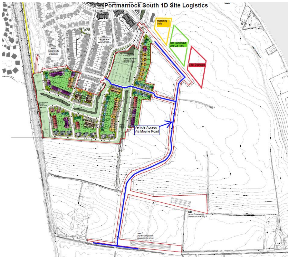
Figure 2.0: Site Logistics
