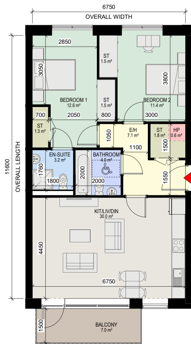
9 Apartment Type 2I 1: 100 - 2 BED, 4 PERSON APARTMENT - GROSS INTERNAL AREA (GIA) : 78.3 sqm
