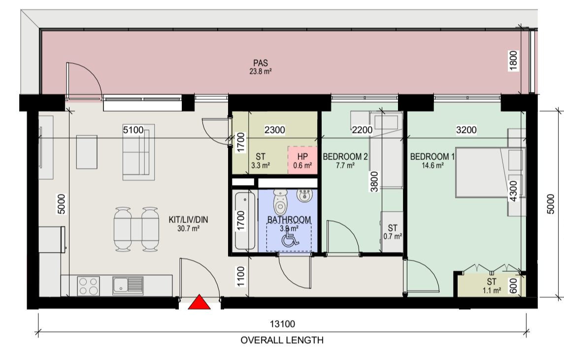
5 Apartment Type 2E 1: 100 - 2 BED, 3 PERSON APARTMENT - GROSS INTERNAL AREA (GIA) : 65.5 sqm
