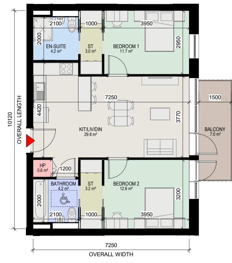
1 Apartment Type 2A 1: 100 - 2 BED, 4 PERSON APARTMENT - GROSS INTERNAL AREA (GIA) : 73.37 sqm
