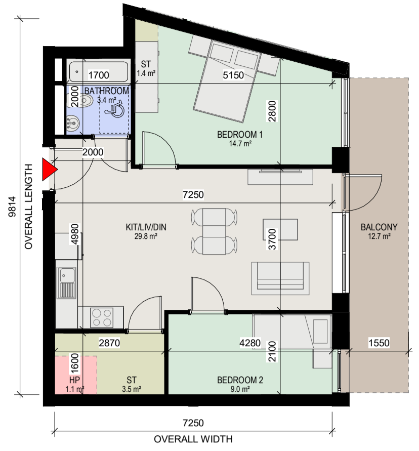
3 Apartment Type 2C 1: 100 - 2 BED, 3 PERSON APARTMENT - GROSS INTERNAL AREA (GIA) : 65.43 sqm
