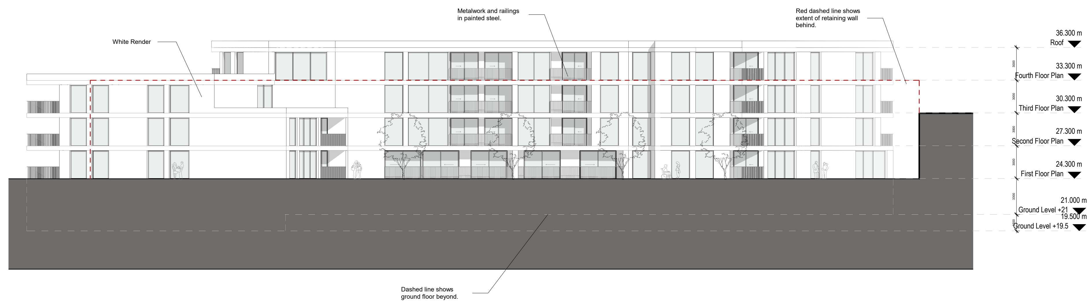
1 Proposed South Elevation 1 : 200
