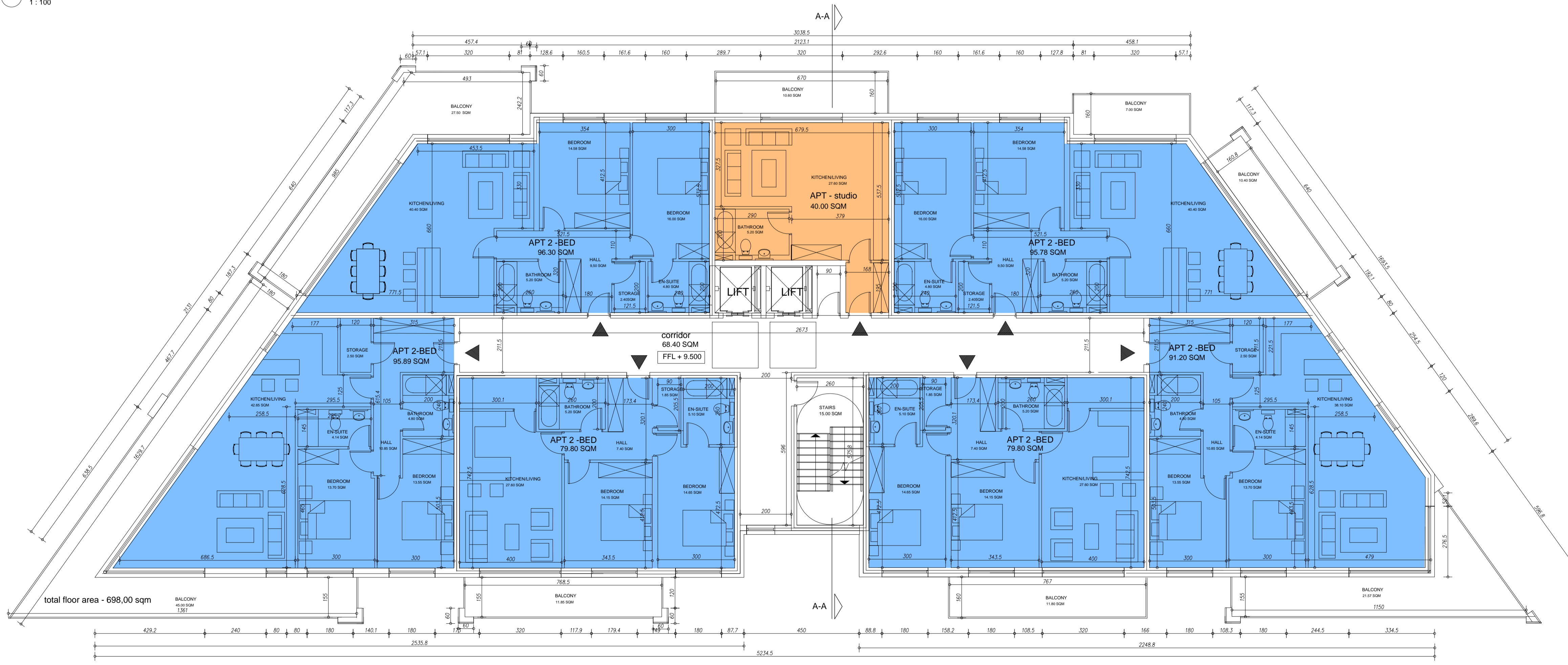
1 PROPOSED BLOCK 2 - 1st-7th FLOOR PLAN 1:100
