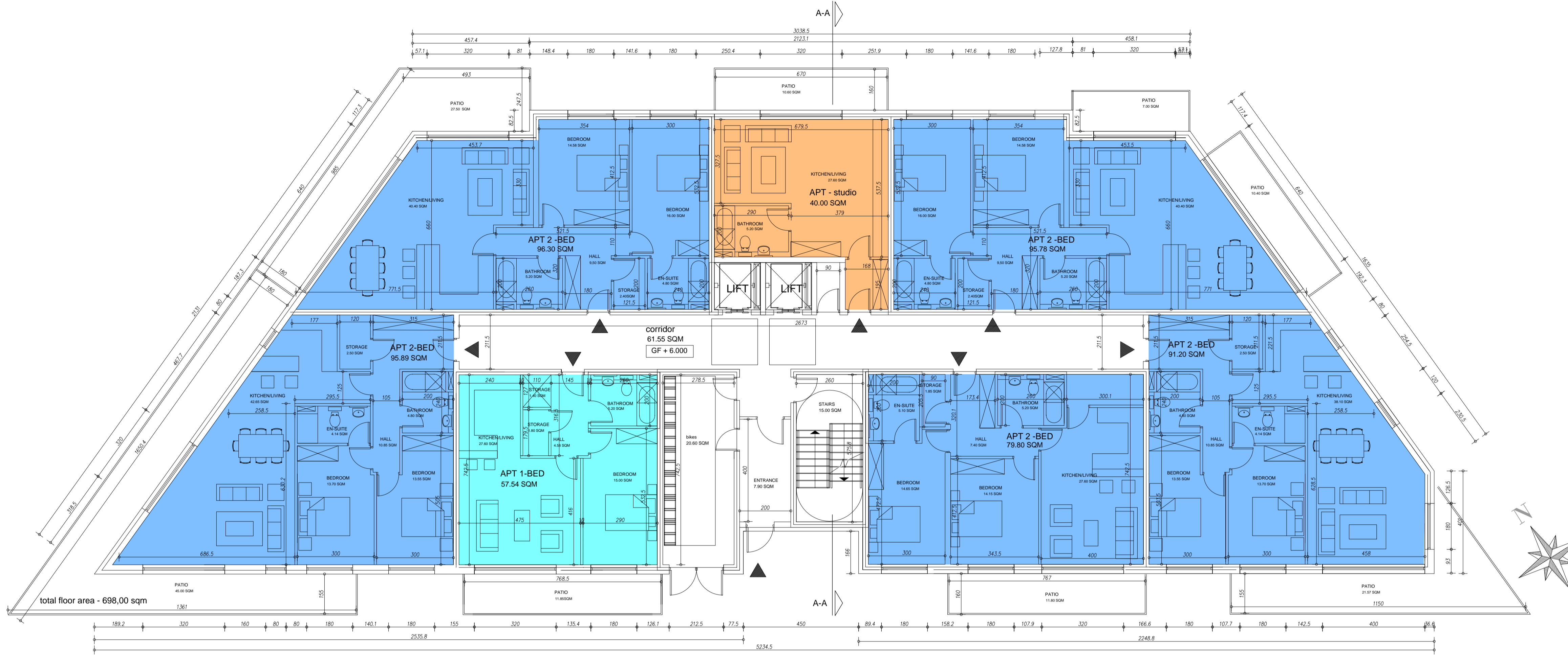
1 PROPOSED BLOCK 2 - GROUND FLOOR PLAN 1:100
