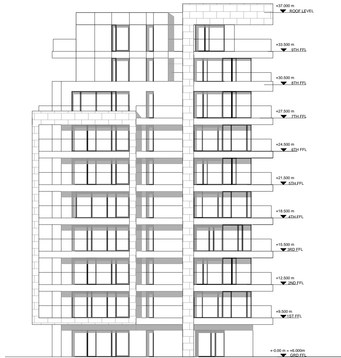
1 PROPOSED BLOCK 2 - SIDE ELEVATION 1 : 200
