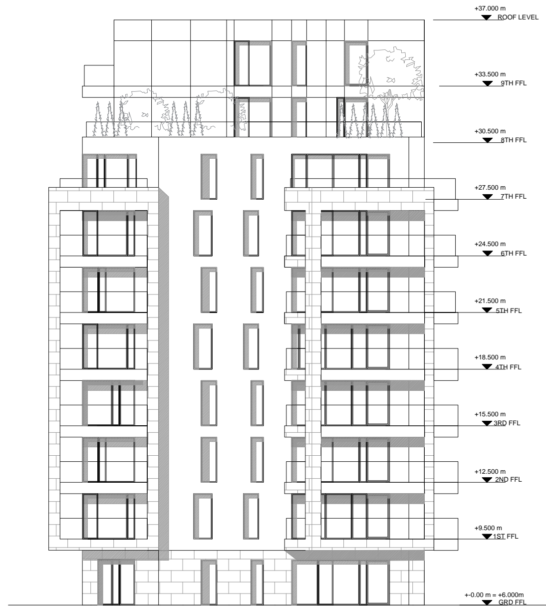
2 PROPOSED BLOCK 2 - SIDE ELEVATION 1 : 200
