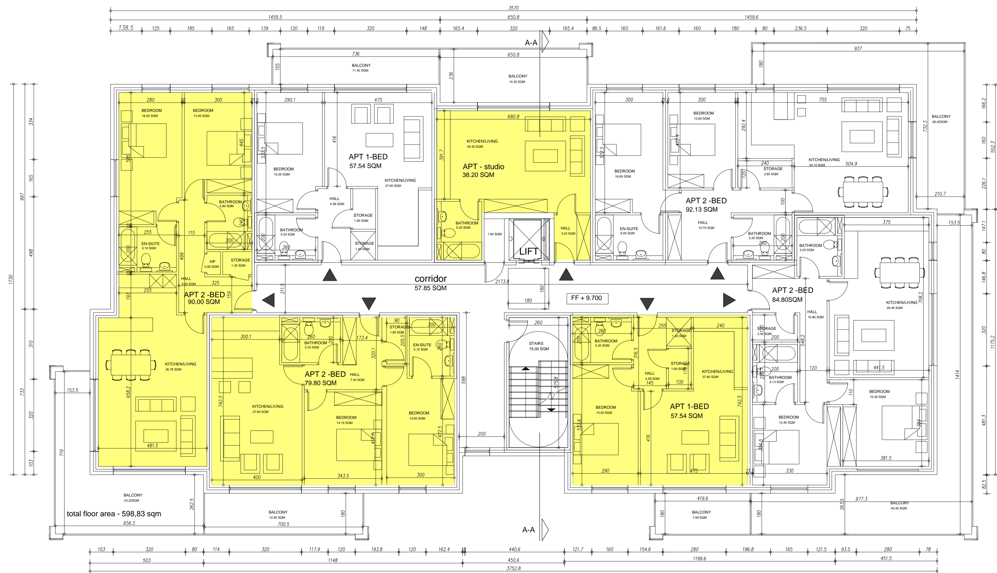
2 PROPOSED BLOCK 4 & 6 - 1st & 2nd FLOOR PLAN 1: 100
