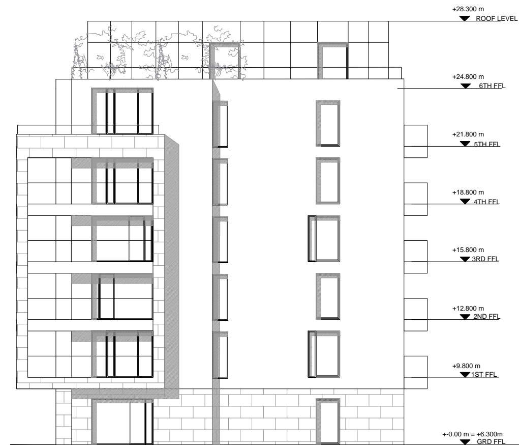
2 PROPOSED BLOCK 5 - SIDE ELEVATION 1 : 200
