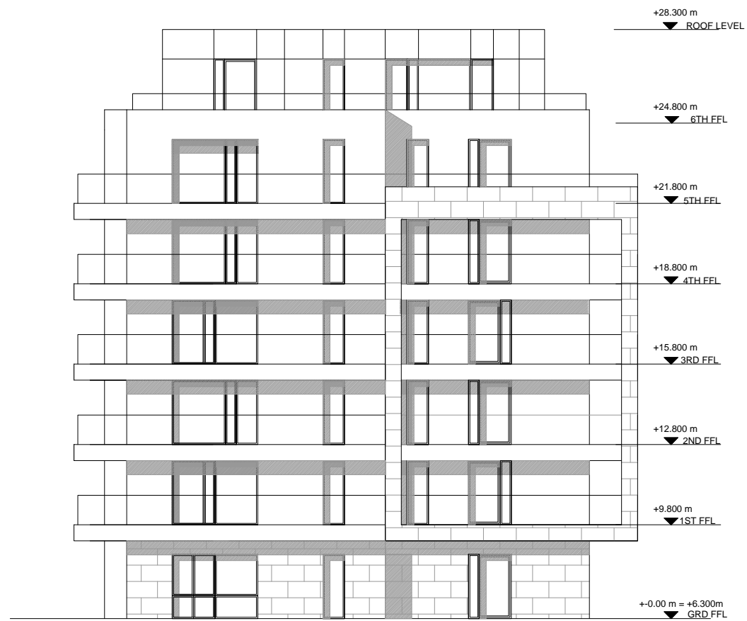
1 PROPOSED BLOCK 5 - SIDE ELEVATION 1 : 200
