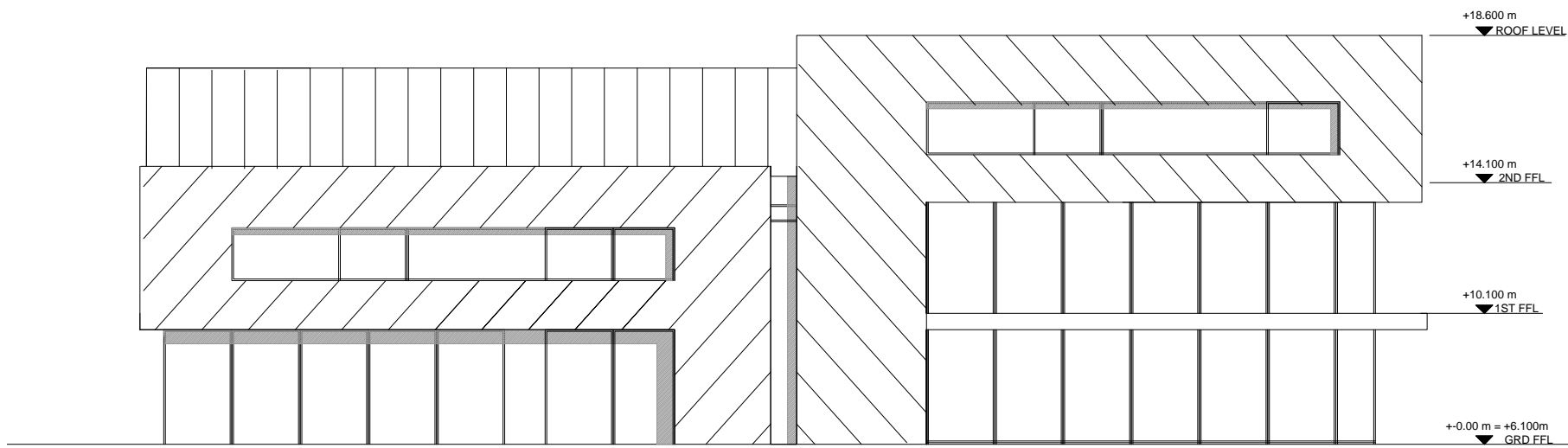
PROPOSED COMMUNITY FACILITIES BUILDING - SIDE ELEVATION
