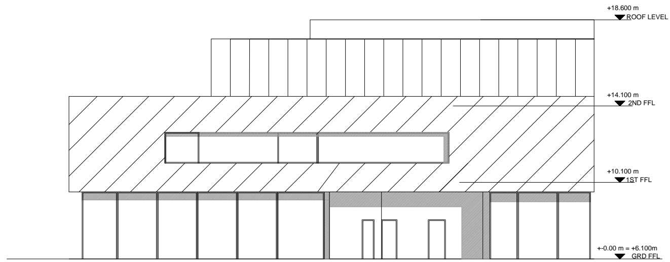
PROPOSED COMMUNITY FACILITIES BUILDING - REAR ELEVATION
