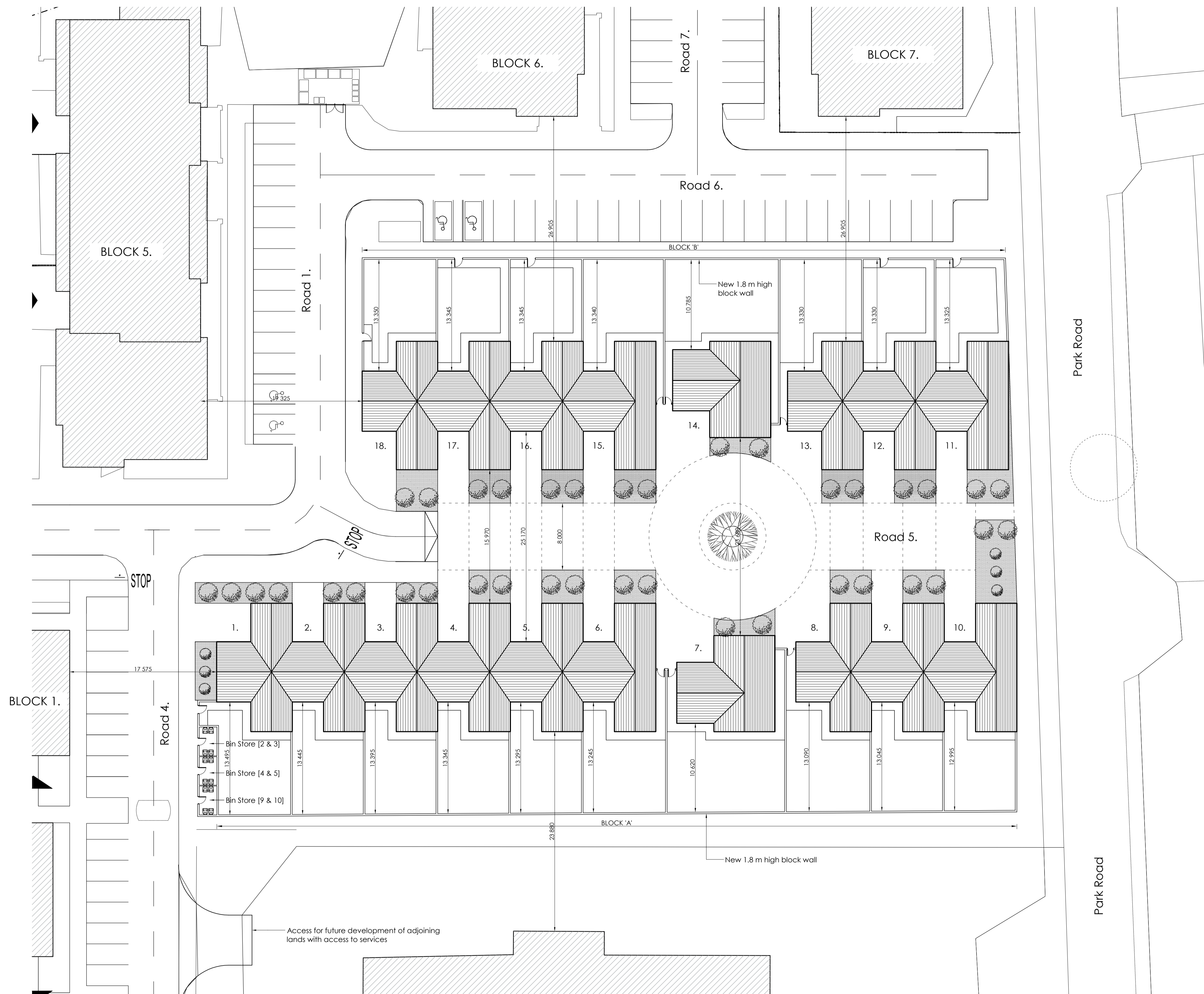
Site Layout Plan Scale 1:250
