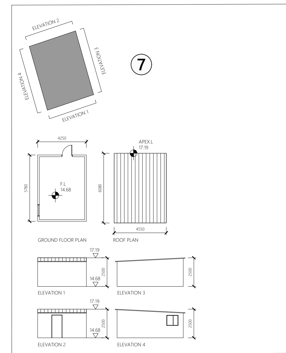
7 BUILDING NO.7 1:200 @ A1
