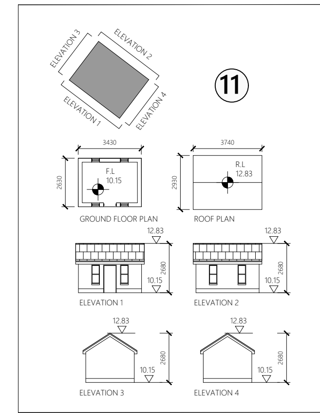
3 BUILDING NO.11 1:200 @ A1
