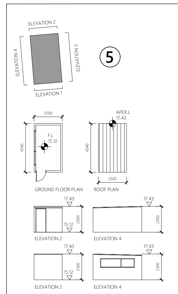
5 BUILDING NO.5 1:200 @ A1
