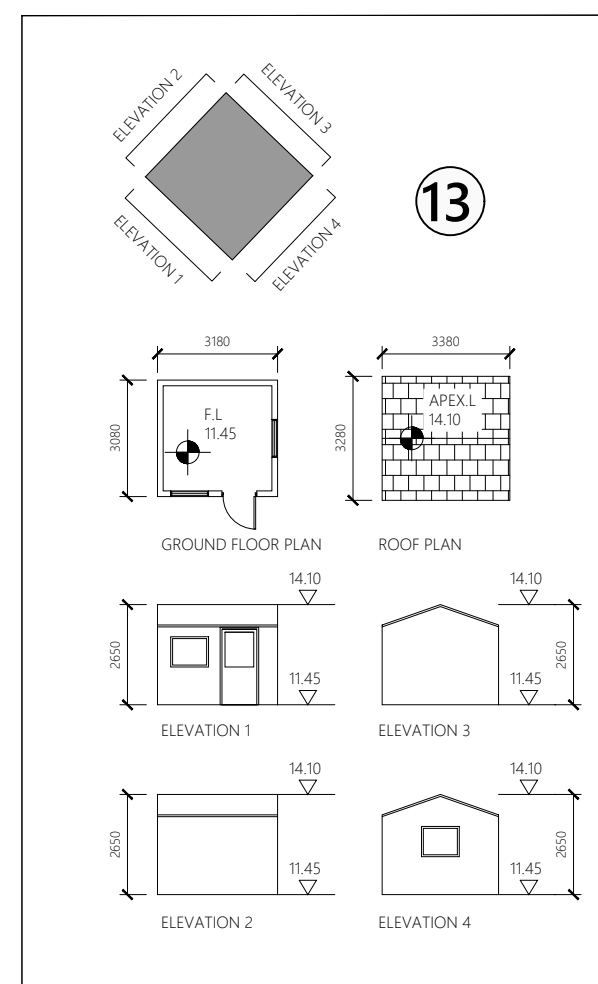
8 BUILDING NO.13 1:200 @ A1
