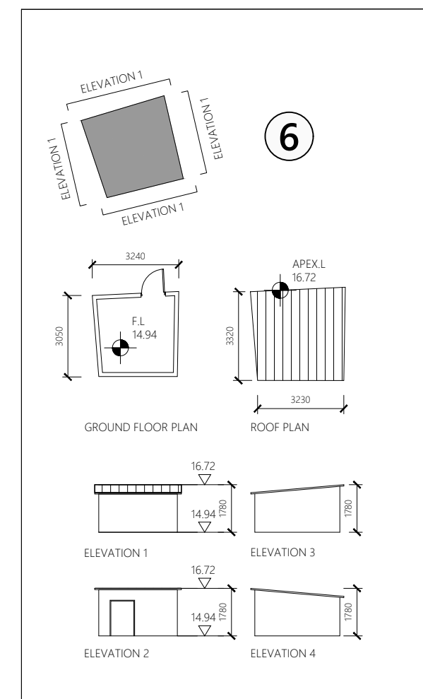
6 BUILDING NO.6 1:200 @ A1
