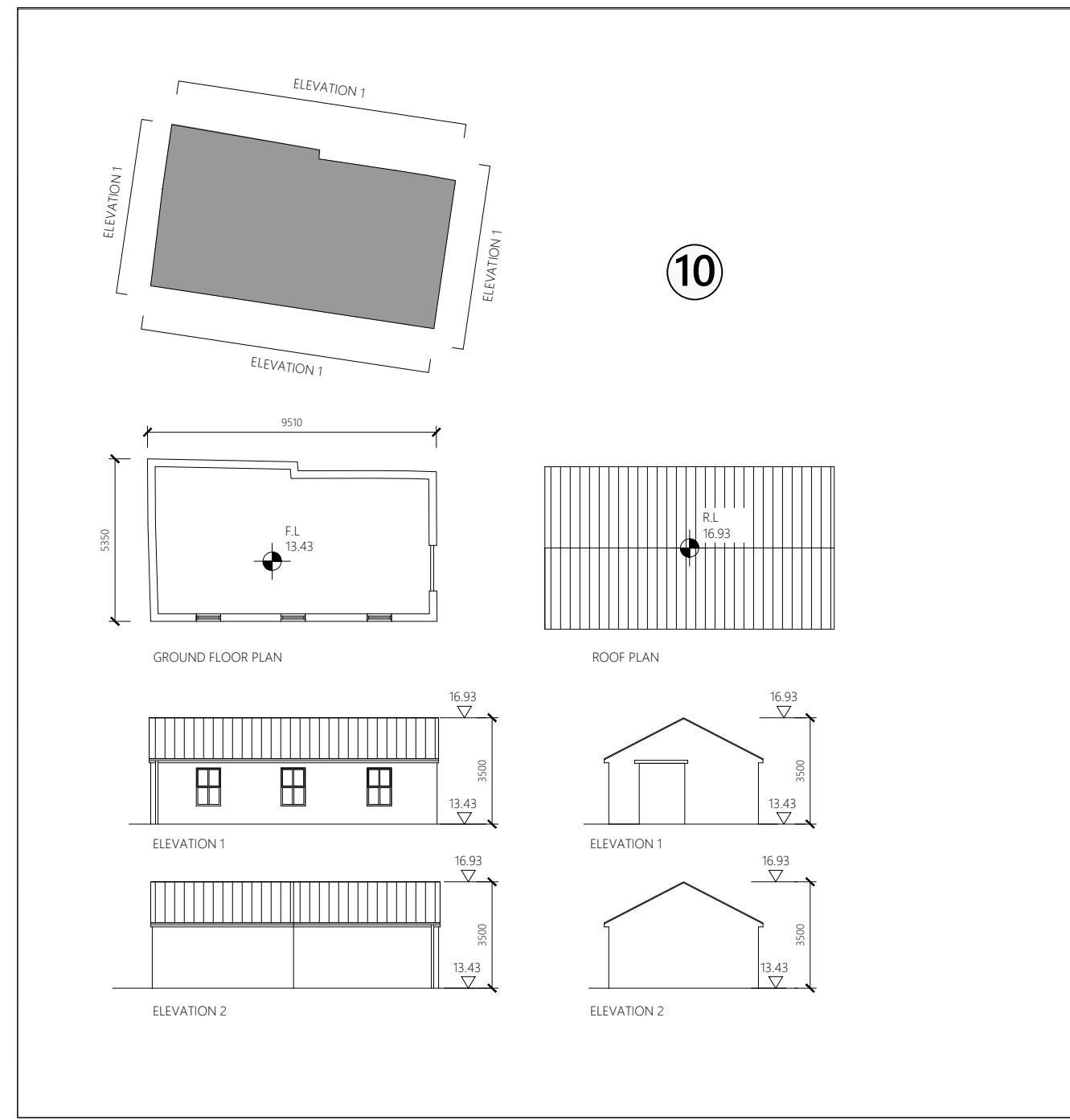
2 BUILDING NO.10 1:200 @ A1
