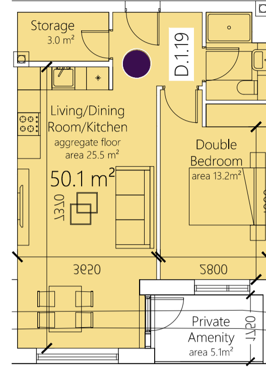
1 BED 2 PERSON i.e. D.0.2, D.0.3, E.0.2, E.0.4 TYPE: 1B2P A1 AREA: 50.1 m 2
