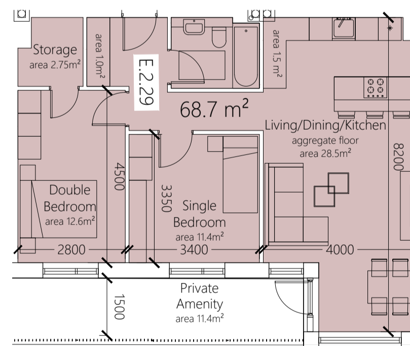
2 BED 3 PERSON i.e. E.2.29 TYPE: 2B3P J AREA: 68.7 m 2
