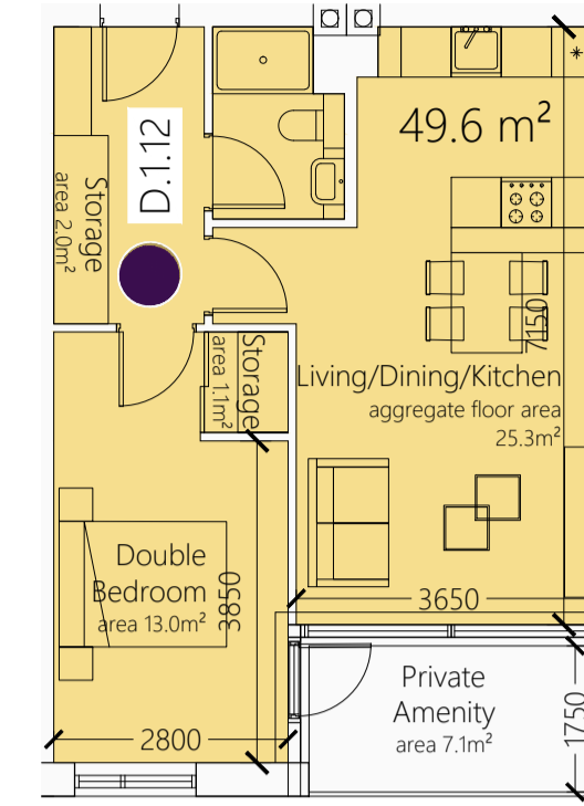
1 BED 2 PERSON i.e. D.1.12, D.2.28, E.1.22, E.2.34 TYPE: 1B2P C1 AREA: 49.6 m 2
