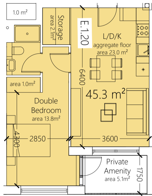
1 BED 2 PERSON i.e. E.1.20, E.2.32, E.3.40 TYPE: 1B2P E AREA: 45.3 m 2
