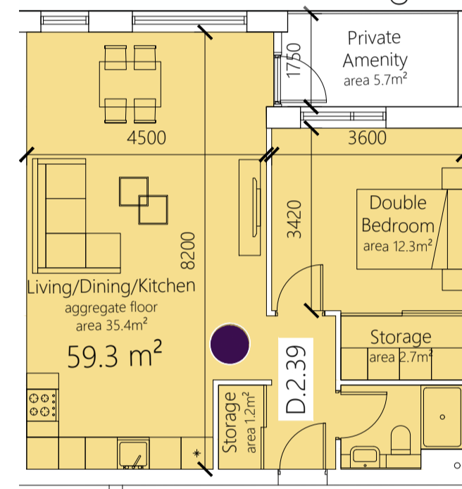
1 BED 2 PERSON i.e. D.2.39, D.3.55 TYPE: 1B2P F AREA: 59.3 m 2
