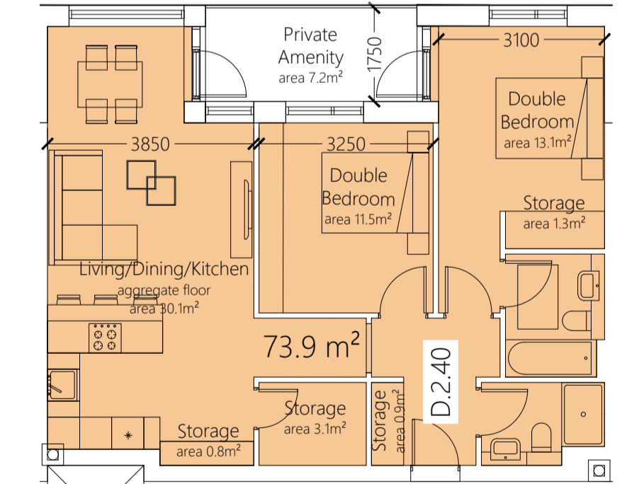
2 BED 4 PERSON i.e. D.2.40, D.3.56, E.1.19, E.2.31 TYPE: 2B4P M AREA: 73.9 m 2
