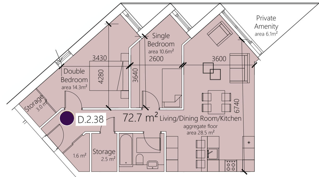
1 BED 2 PERSON i.e. D.1.21, D.2.38, D.3.54 TYPE: 2B3P I AREA: 72.7 m 2
