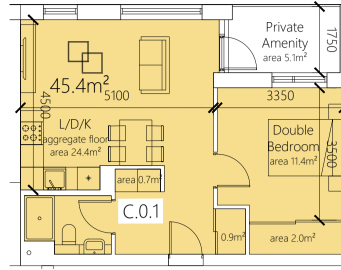
1 BED 2 PERSON i.e. C.0.1, C.1.11, C.2.23 TYPE: 1B2P B AREA: 45.4 m 2
