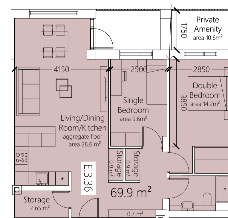
2 BED 3 PERSON i.e. E.3.36, E.4.44 TYPE: 2B3P K AREA: 69.9 m 2
