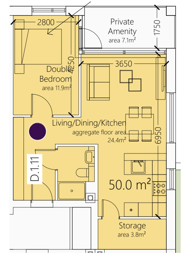
1 BED 2 PERSON i.e. D.1.11, D.2.27 TYPE: 1B2P D AREA: 50.0 m 2
