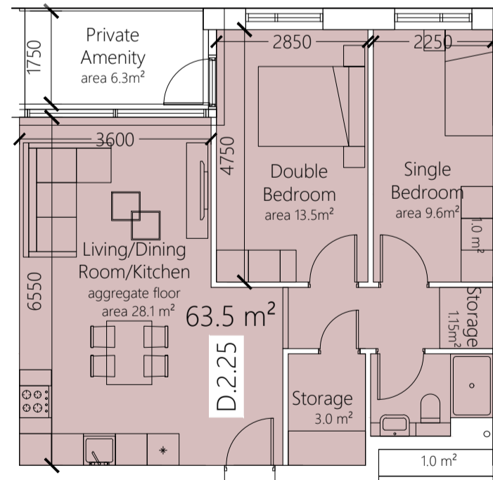
2 BED 3 PERSON i.e. D.1.9, D.2.25, D.3.43 TYPE: 2B3P H AREA: 63.5 m 2
