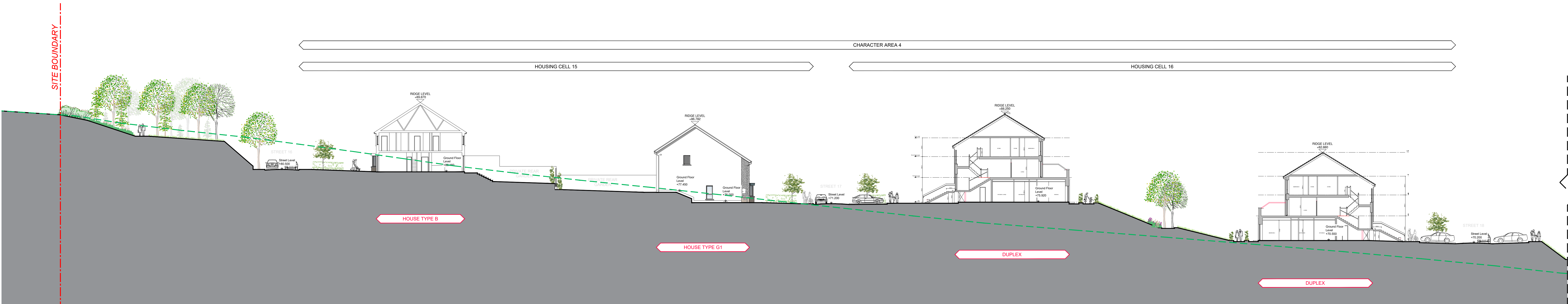
SECTION E-E (PART 1) - CHARACTER AREA 4 Scale 1:200
