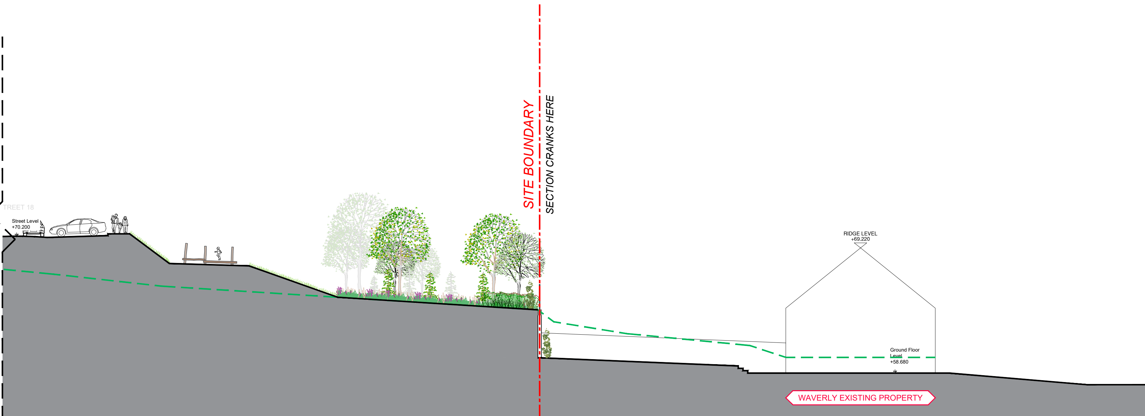
SECTION E-E (PART 2) - CHARACTER AREA 4 Scale 1:200
