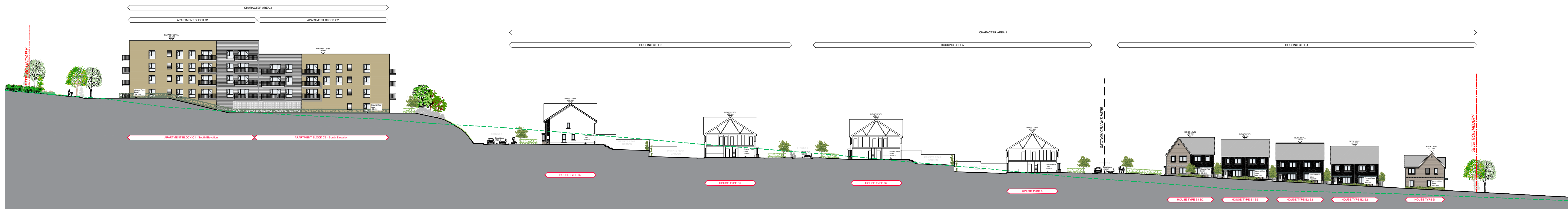
SECTION F-F - CHARACTER AREA 2 + 1 Scale 1:500
