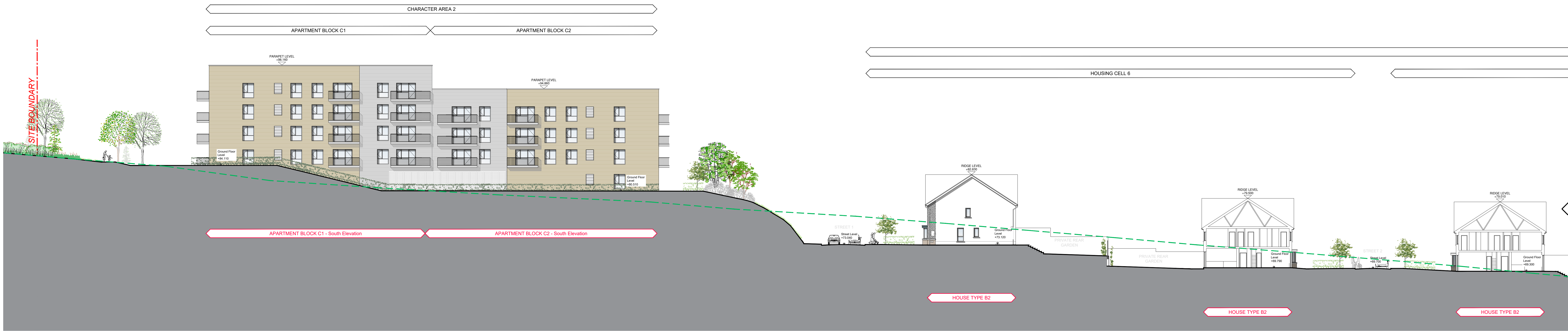
SECTION F-F (PART 1) - CHARACTER AREA 2 + 1 Scale 1:200
