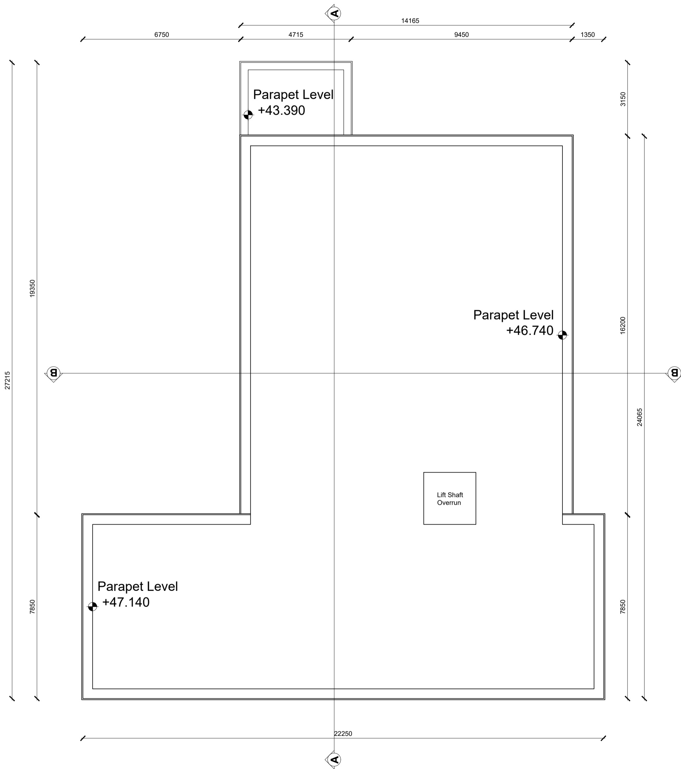
CRECHE ROOF PLAN
