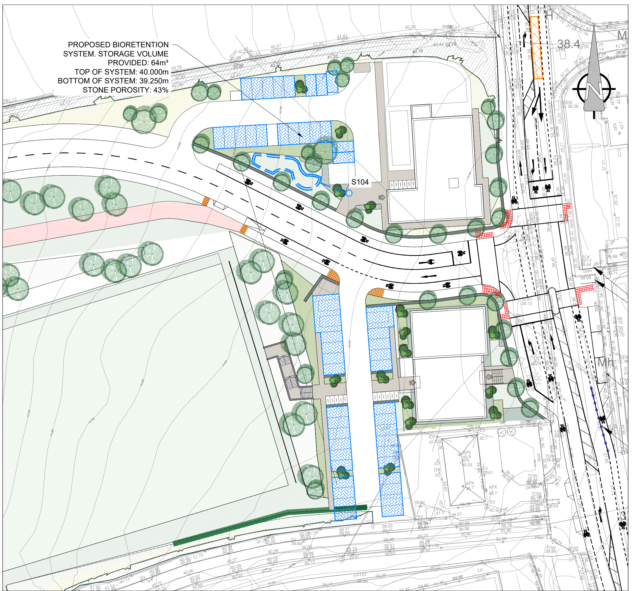
B PROPOSED SuDS MEASURES - SHEET 4 OF 4 0524 Scale: 1:500
