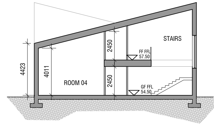
SECTION CR SCALE 1:200
