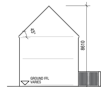
SIDE ELEVATION D3 SCALE 1:200
