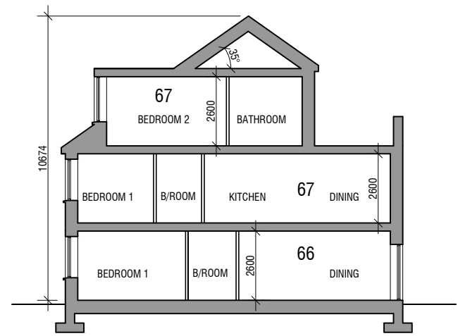
SECTION SCALE 1:200
