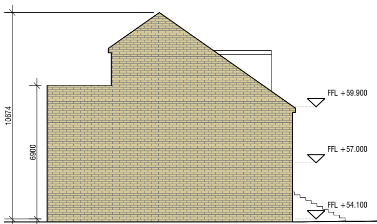
LHS ELEVATION - TYPE E1.1 SCALE 1:200
