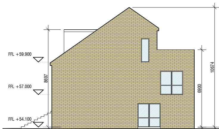
RHS ELEVATION - TYPE E1.1 SCALE 1:200
