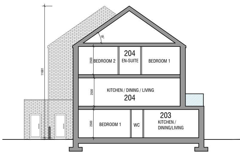
SECTION SCALE 1:200
