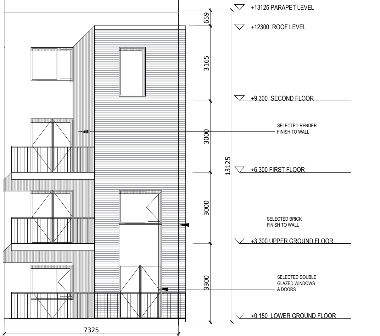
North Elevation to Park 1:100
